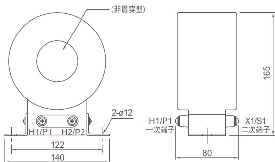
FIG.1 CG-P5 (繞線型)
