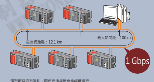
[環型拓撲]
