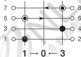
CS (1a-0-1a, 附1a+1b 殘留接點)
