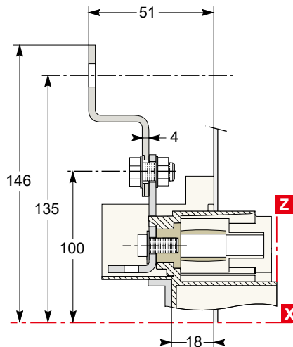
CVS100 to 250
