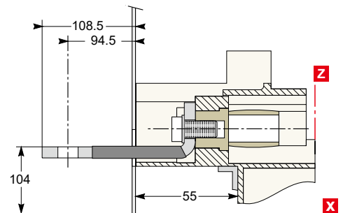
CVS400 to 630
