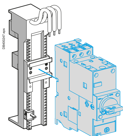
Installation examples.
