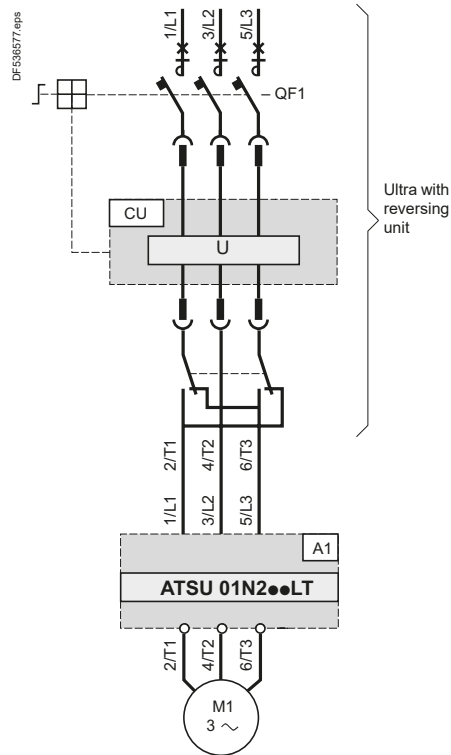
Power wiring with reversing unit
