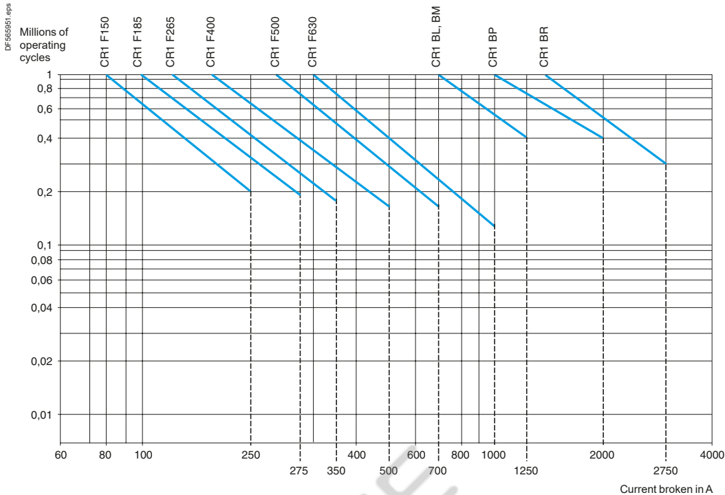
Electrical durability (Ue ≤ 440 V) (1)
