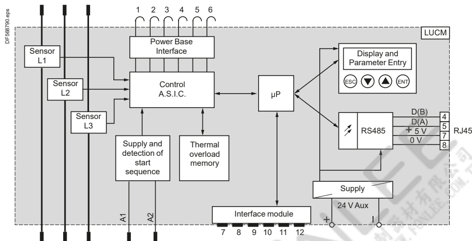
Basic scheme
