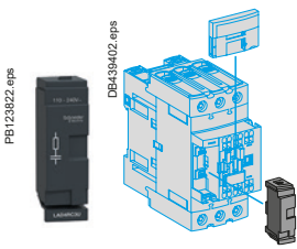
LAD4RC3●, LAD4V3●, LAD4D3U, LAD4T3●
