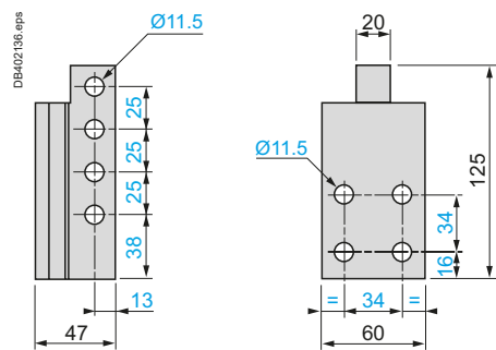
Right-angled connectors LA9F2100 (set of 6) for rear connection
