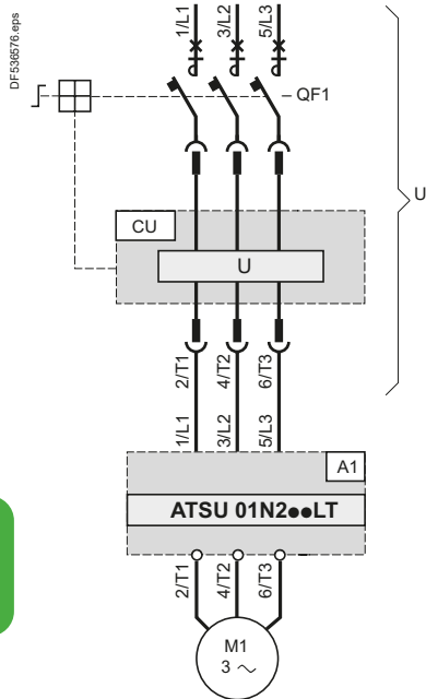
Power wiring
