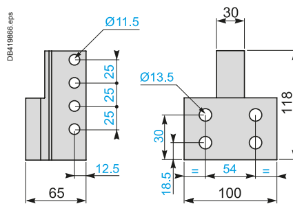
Right-angled connectors LA9F2600 (set of 6) for rear connection
