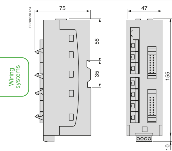
Parallel RJ45 wiring modules Splitter box LU9G02
