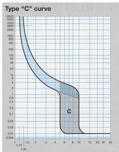
Characteristic curve
