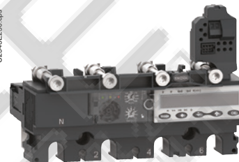
MicroLogic trip units for 3 poles, 4 poles ComPacT circuit breakers
