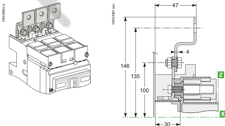
NSX100 to 250
