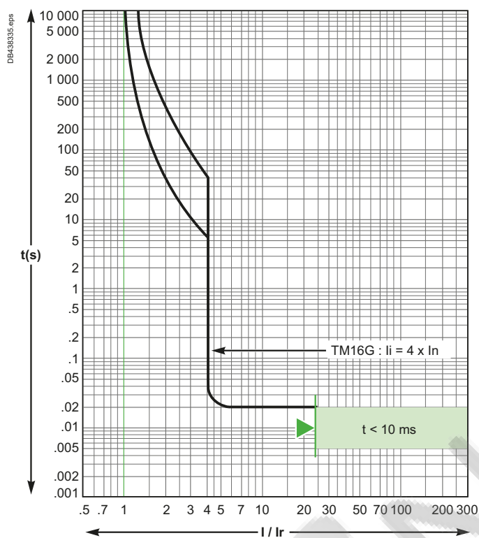
TM16G
