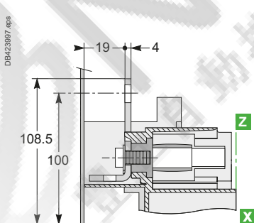
NSX100 to 250
