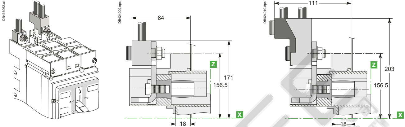
NSX400/630
