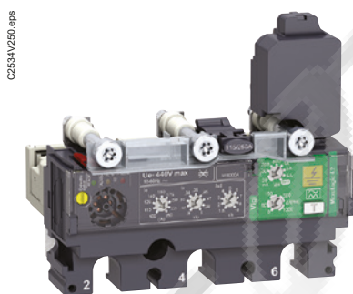
MicroLogic Vigi 4 (LS 0 IR)
