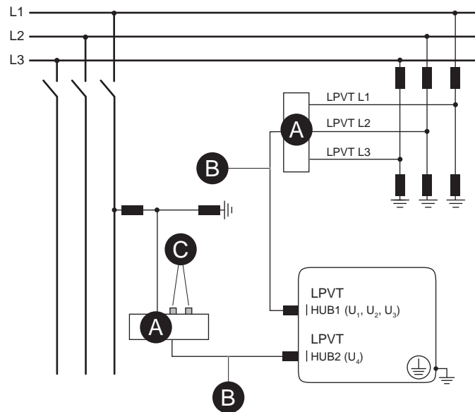
Figure 218 - Three line-to-neutral LPVTs + one line-to-neutral LPVT
