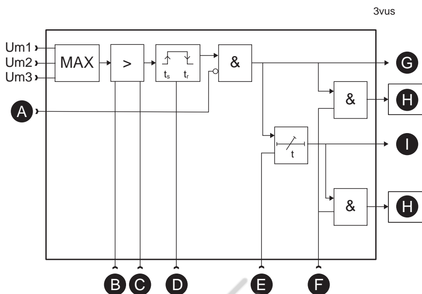
Figure 106 - Block diagram of the three-phase overvoltage stages U>, U>> and U>>>
