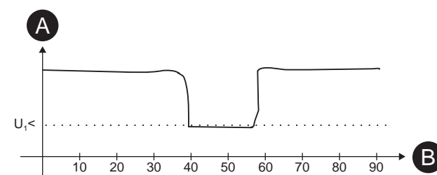
Figure 137 - A short voltage interruption which is probably not recognized
