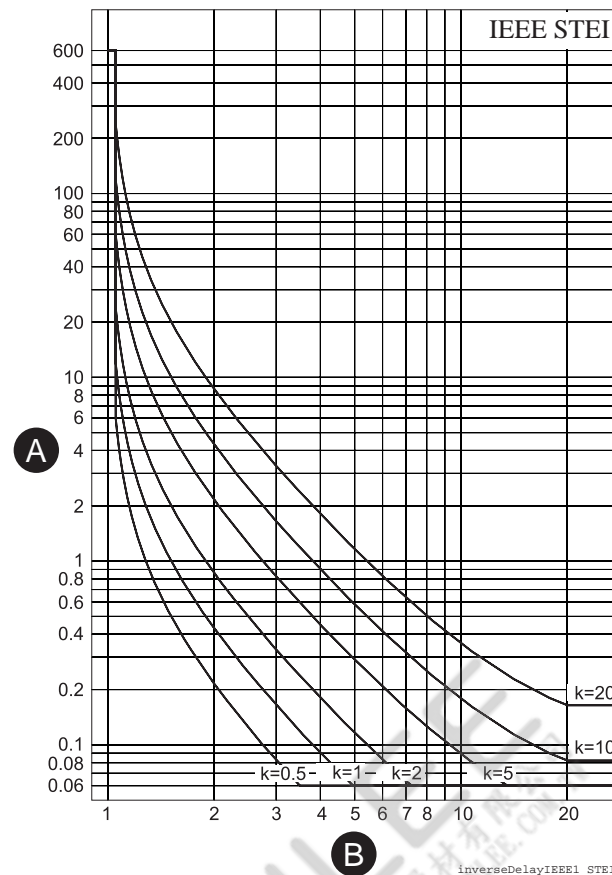
Figure 64 - ANSI/IEEE short time extremely inverse delay
