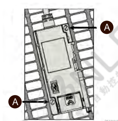
Figure 228 - Mounting on Telequick grid
