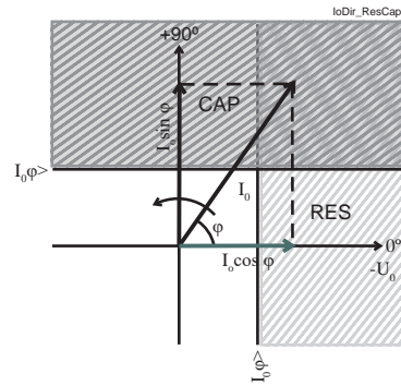
Figure 115 - Operation characteristics of the directional earth fault protection in Res and Cap mode
