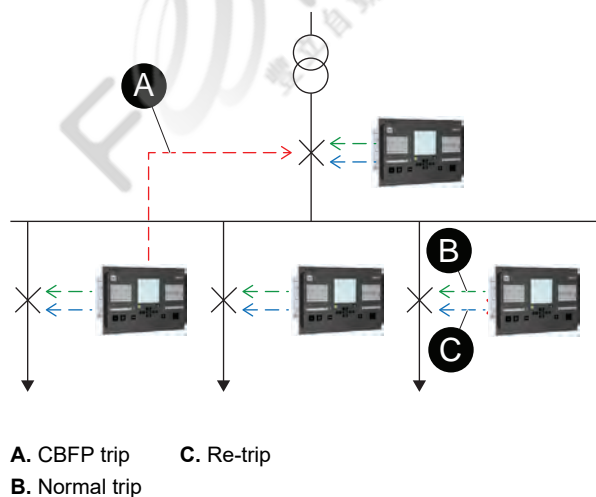
Figure 85 - CBFP implementation
