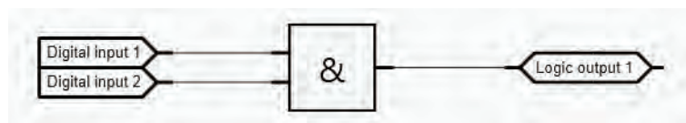
Figure 161 - An example of logic configuration for trip circuit supervision with two digital inputs DI1 and DI2.
