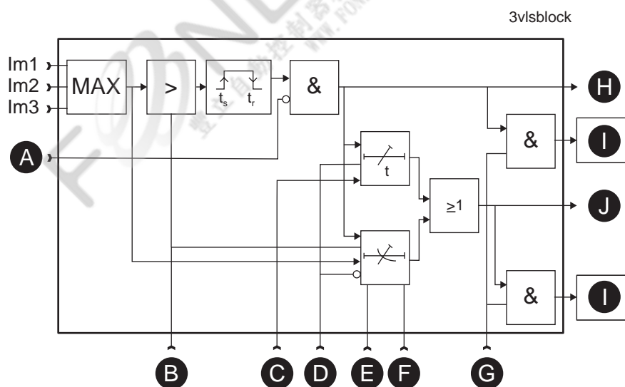
Figure 91 - Block diagram of the three-phase overcurrent stage I >
