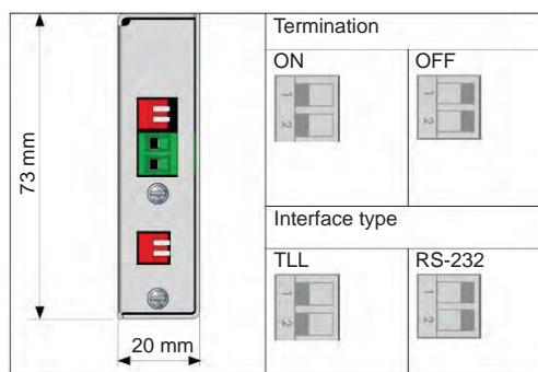
Figure 195 - RS-232 and TTL interface
