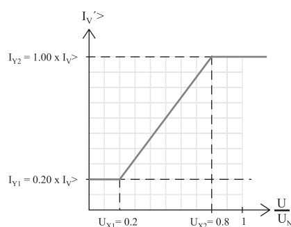
Figure 104 - Characteristics of the voltage-restrained overcurrent function I_V>
