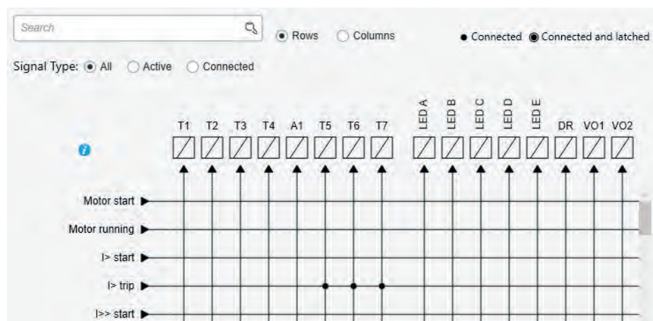
Figure 16 - Output matrix view
