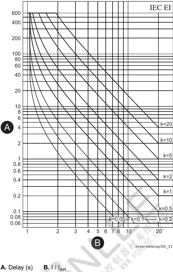
Figure 56 - IEC extremely inverse delay
