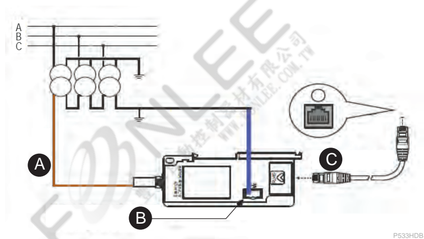
Figure 224 - Open-delta connection 2
