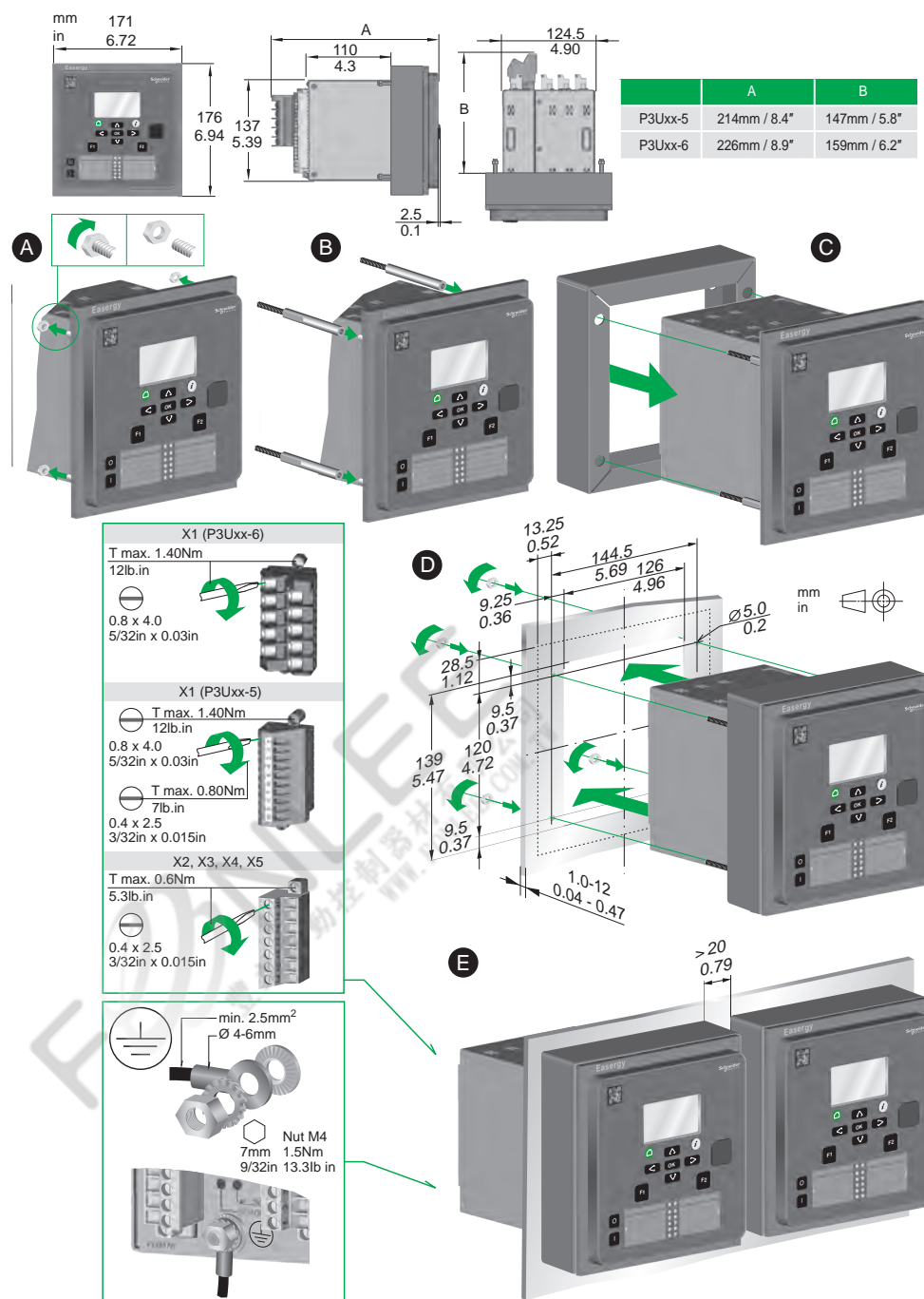
Figure 184 - Panel mounting with the raising frame REL52834
