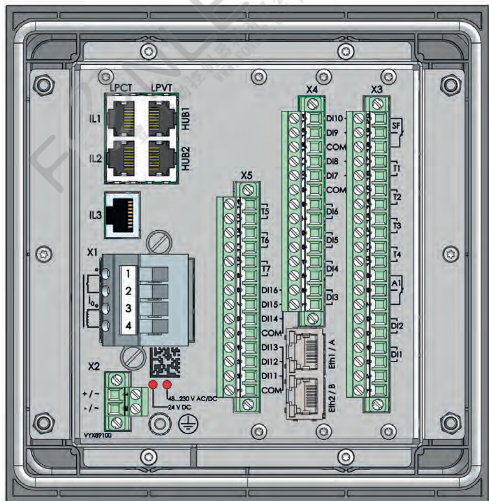
Figure 219 - P3U rear panel – LPIT
