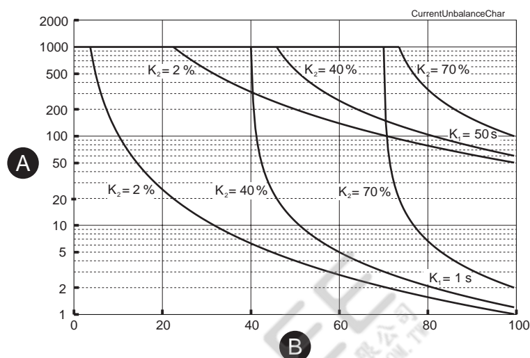
Figure 75 - Dependent operation delay of negative sequence overcurrent I_2 > (ANSI 46). The longest delay is limited to 1000 seconds (=16min 40s).
