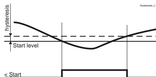
Figure 53 - Example behavior of an under-protection with hysteresis
