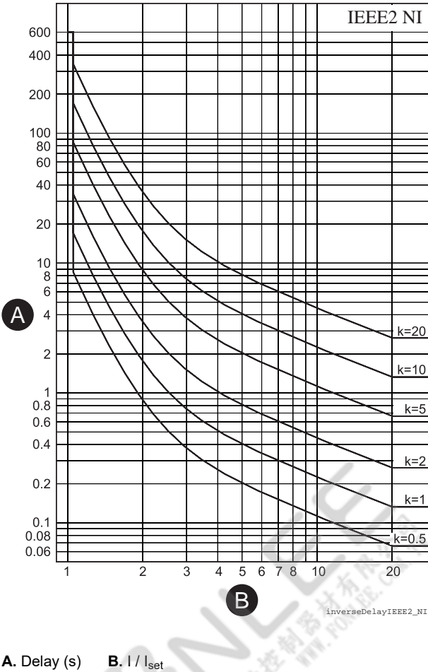
Figure 66 - IEEE2 normal inverse delay
