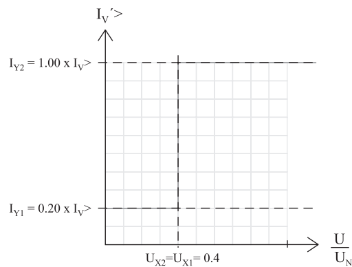
Figure 105 - Voltage-controlled overcurrent characteristics
