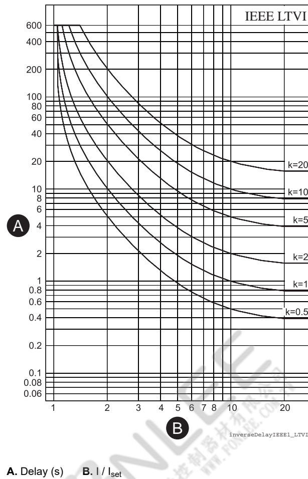
Figure 60 - ANSI/IEEE long time very inverse delay
