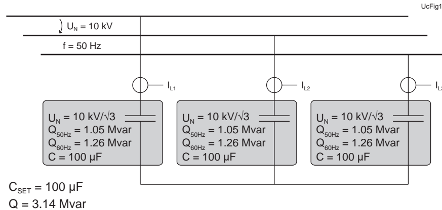
Figure 107 - Capacitor bank built of three single-phase units connected in wye (III Y). Each capacitor is 100 \mu\text{F} and this value is also used as the setting value.
