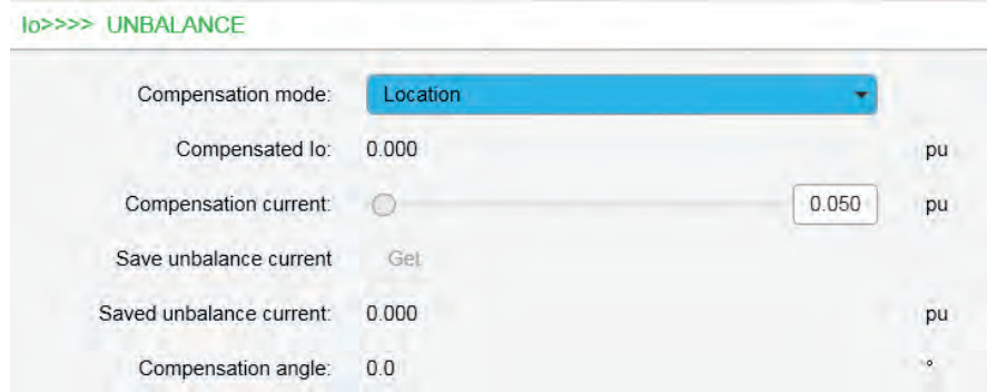
Figure 99 - Enabling unbalance protection
