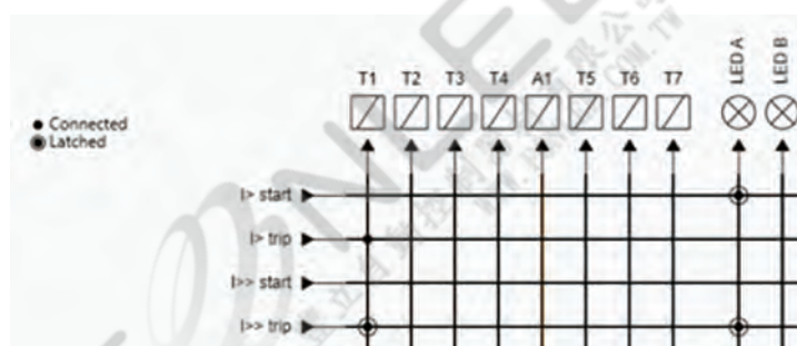
Figure 129 - The lockout programmed for LED A and I>> trip signals
