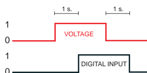
Figure 20 - Digital input's behavior when delay is set to 1 second
