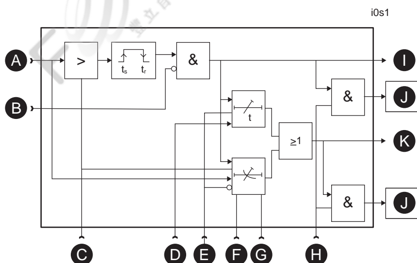
Figure 93 - Block diagram of the earth fault stage overcurrent I_0 >
