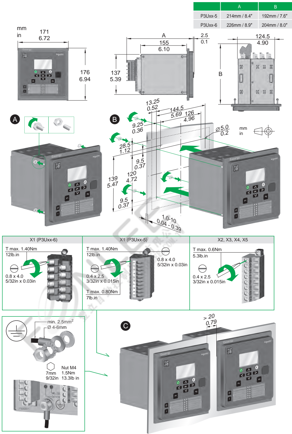
Figure 183 - Panel mounting
