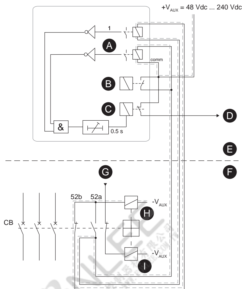
Figure 159 - Trip circuit supervision with two digital inputs and CB in open position
