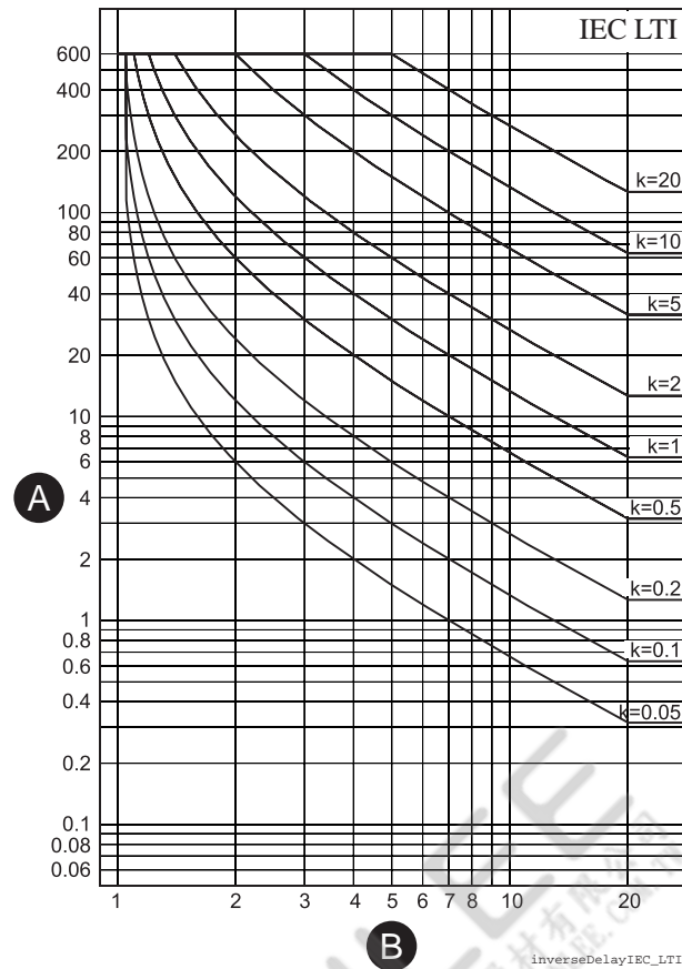
Figure 58 - IEC long time inverse delay
