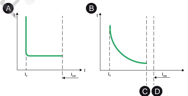
Figure 43 - Overcurrent characteristics
