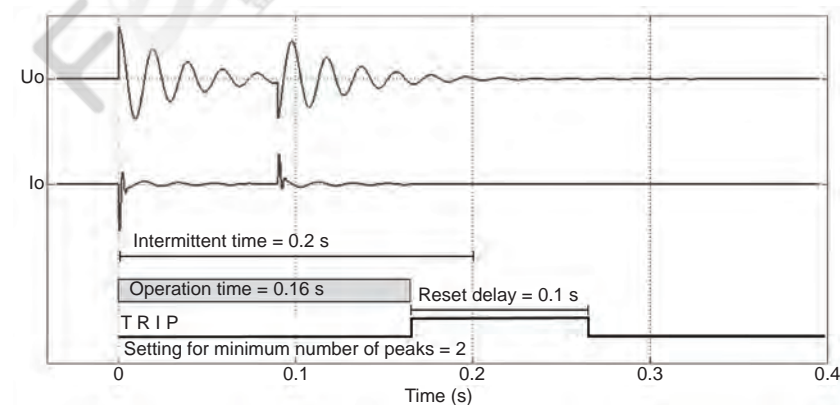
Figure 118 - Set peak amount is satisfied and operate time comes full inside intermittent time setting. Stage issues a trip.
