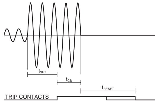
Figure 51 - Reset time
