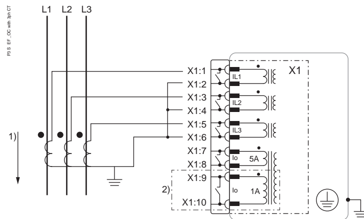
Figure 208 - Three-phase current measurement and summation of earth fault overcurrent
