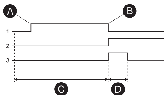
Figure 73 - Synchrocheck function principle
