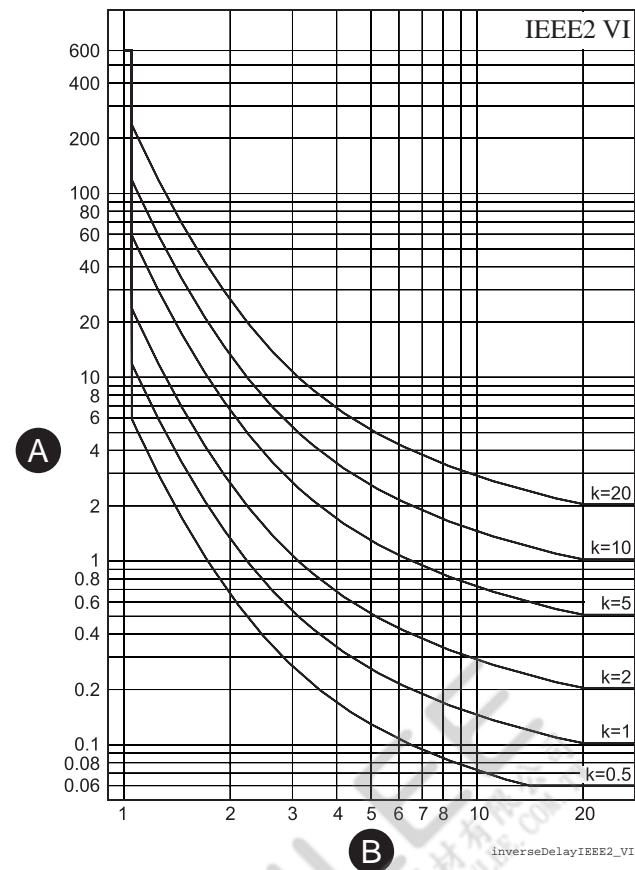
Figure 67 - IEEE2 very inverse delay
