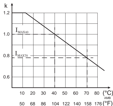
Figure 82 - Ambient temperature correction of the overload stage T>
