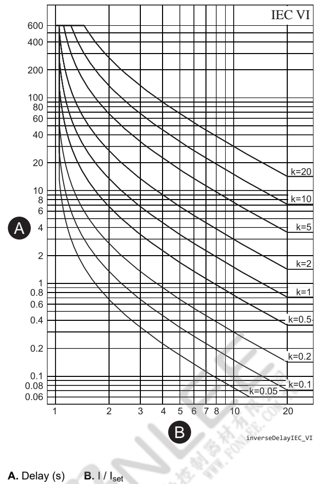
Figure 57 - IEC very inverse delay
