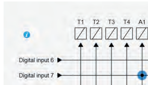
Figure 157 - Example of output matrix configuration for trip circuit supervision with one digital input
