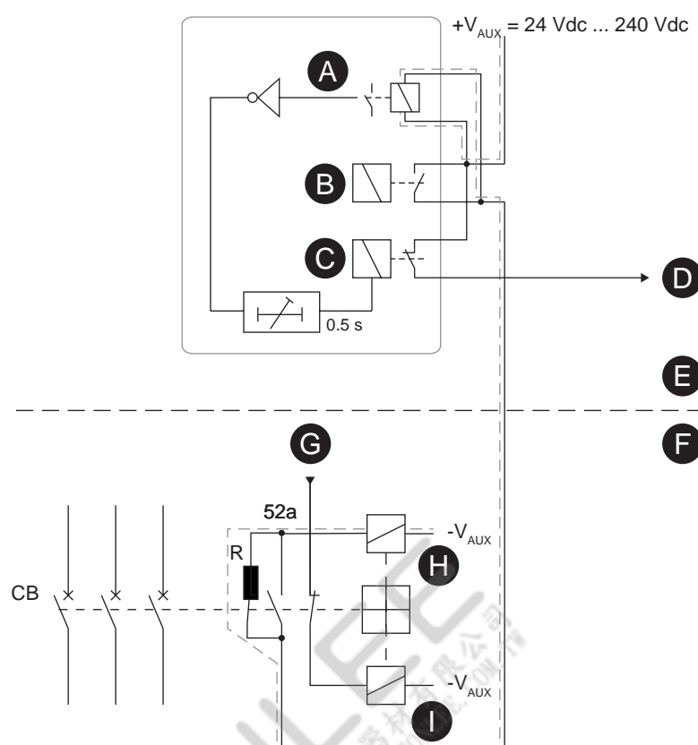
Figure 155 - Alternative connection without using circuit breaker 52b auxiliary contacts. Trip circuit supervision using a single digital input, when the circuit breaker is in open position
