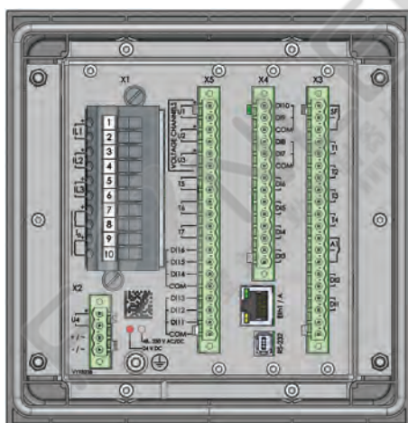
Figure 187 - Pluggable Clamp RJ45 ETH_RS232 without X2-X5 connectors P3Uxx-5ABA1BEA
