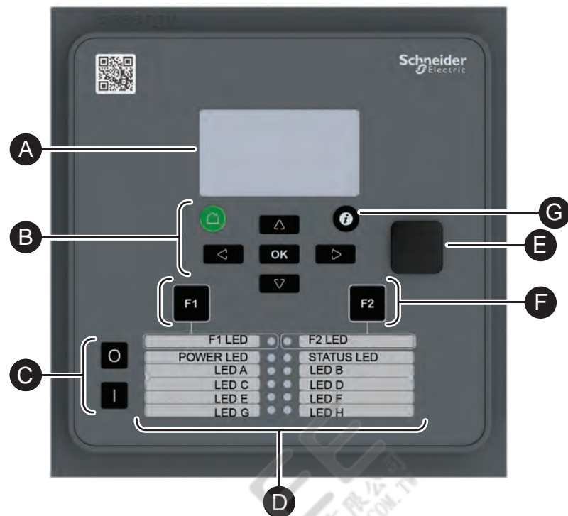
Figure 2 - Easergy P3U10, P3U20 and P3U30 front panel
