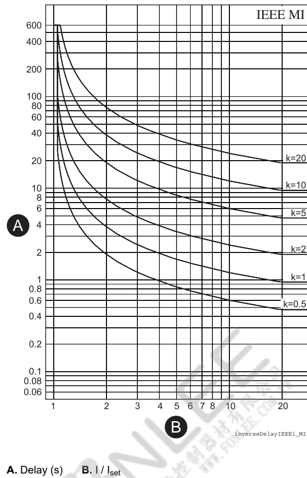
Figure 62 - ANSI/IEEE moderately inverse delay
