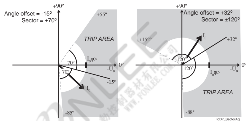
Figure 116 - Operation characteristics examples of the directional earth fault stages in the sector mode
