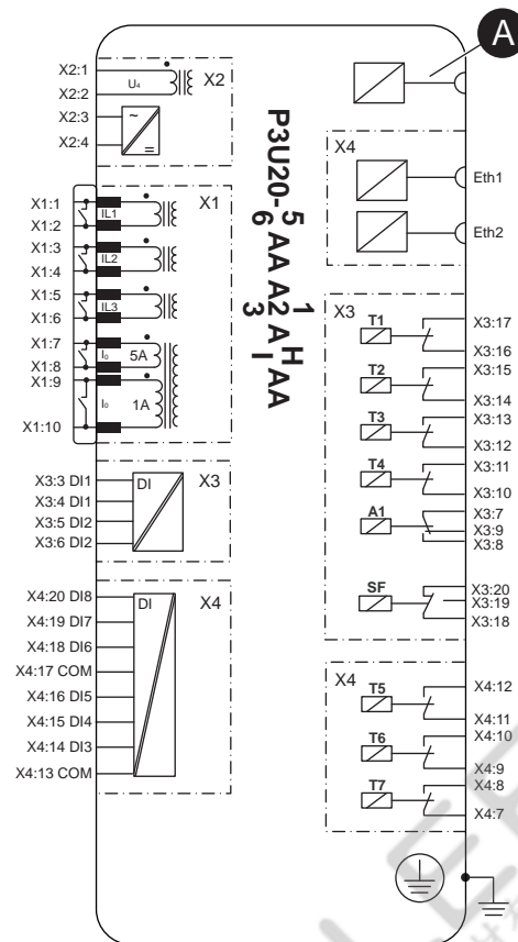
Figure 200 - P3U20 5AA A1AHAA block diagram
