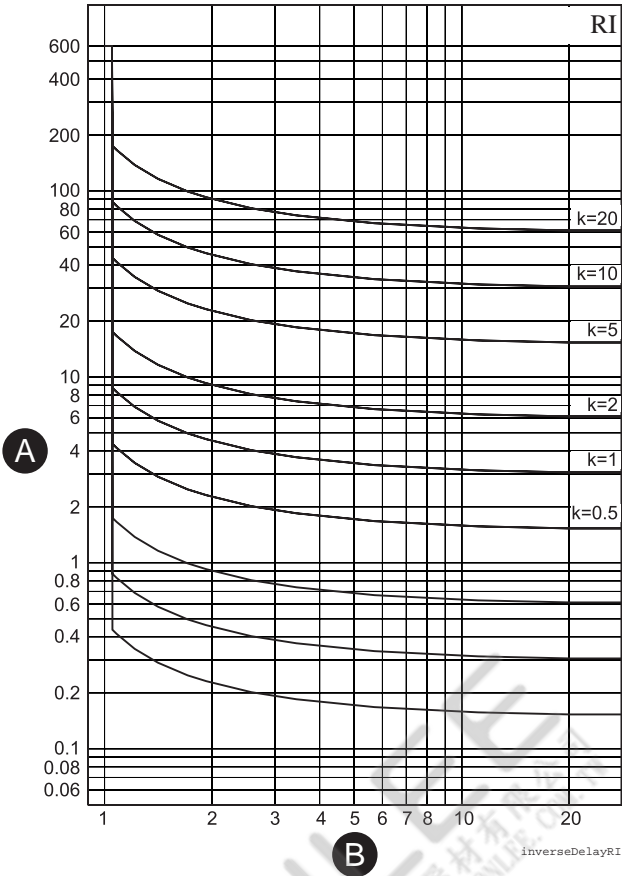
Figure 69 - RI dependent delay
