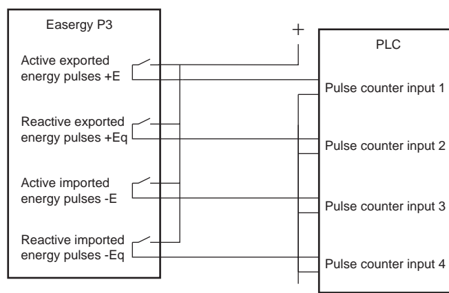
Figure 146 - Application example of wiring the energy pulse outputs to a PLC having common minus and using an external wetting voltage
