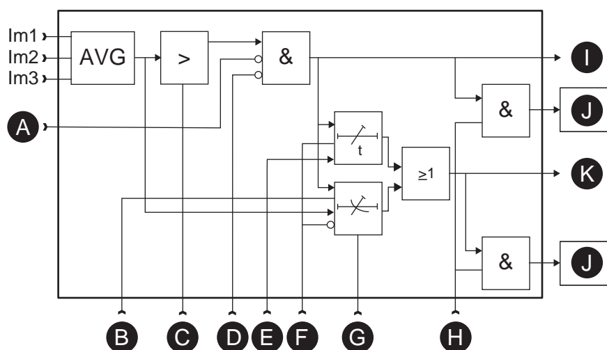
Figure 103 - Block diagram of the locked rotor protection stage I_{lr}
