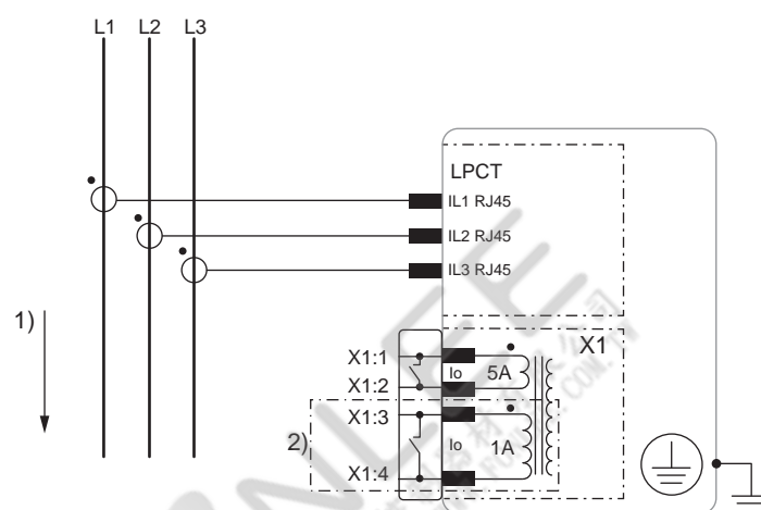
Figure 216 - Three-phase current measurement with LPCTs
