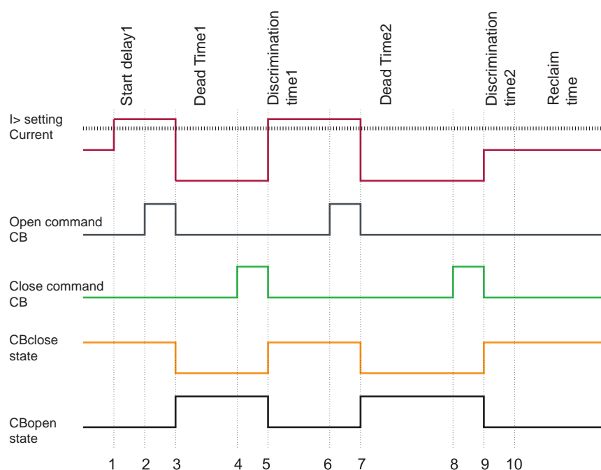
Figure 124 - Example sequence of two shots. After shot 2, the fault is cleared.
