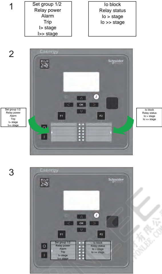
Figure 185 - Example of the P3U alarm facial label insertion
