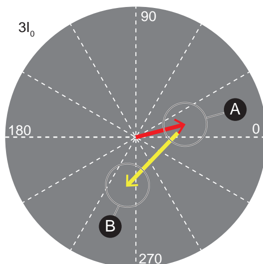
Figure 96 - Natural unbalance compensation and a single capacitor fault
