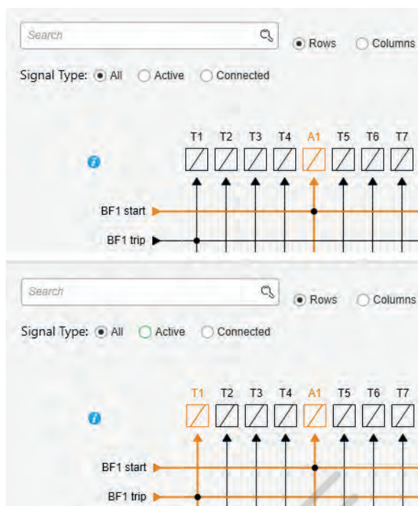
Figure 84 - Trip and CBFP start signals in the Output matrix view
