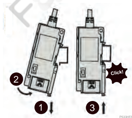
Figure 226 - Mounting on DIN rail
