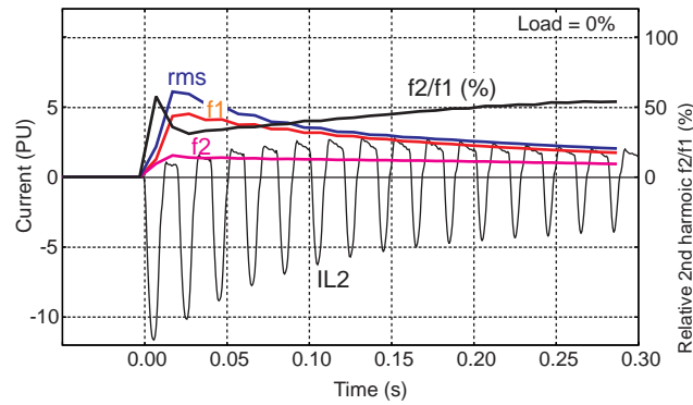
Figure 6 - Example of various current values of a transformer inrush current
