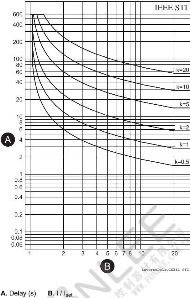
Figure 63 - ANSI/IEEE short time inverse delay
