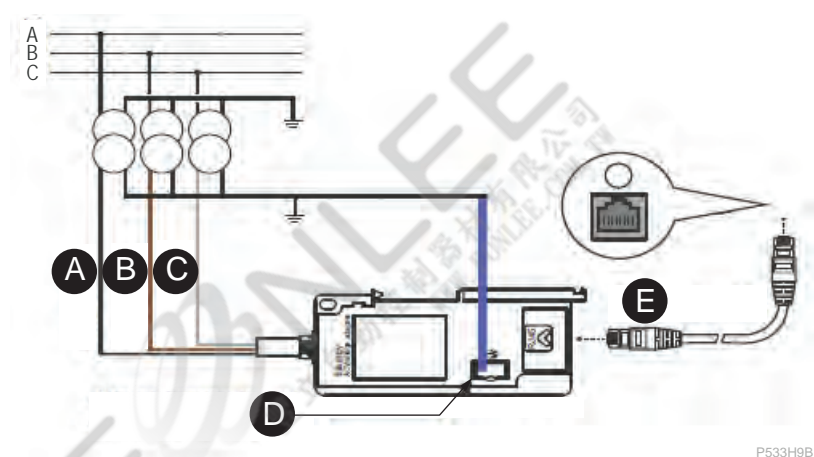
Figure 220 - 3 phase-to-neutral voltages connection
