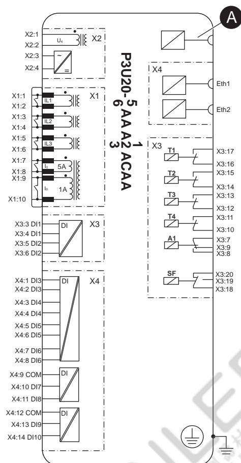
Figure 199 - P3U20 5AA A1ACAA block diagram
