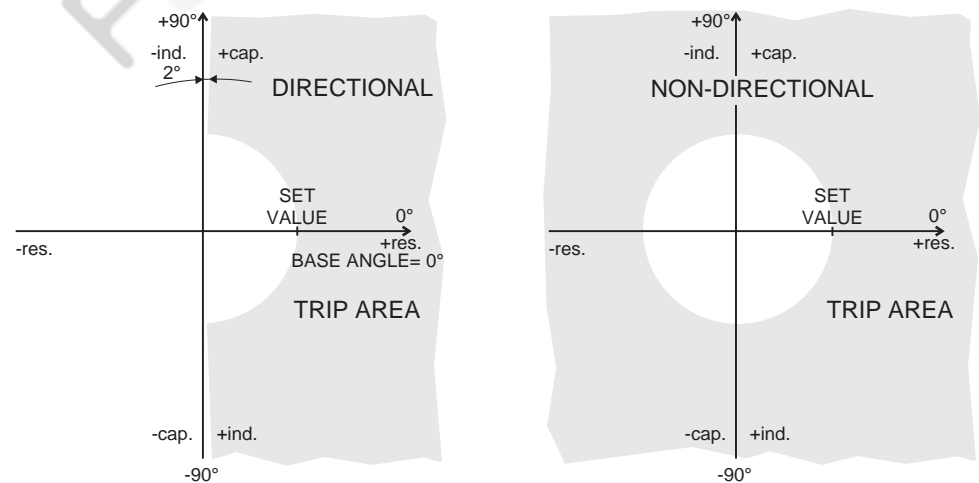
Figure 112 - Difference between directional mode and non-directional mode. The grey area is the trip region.
