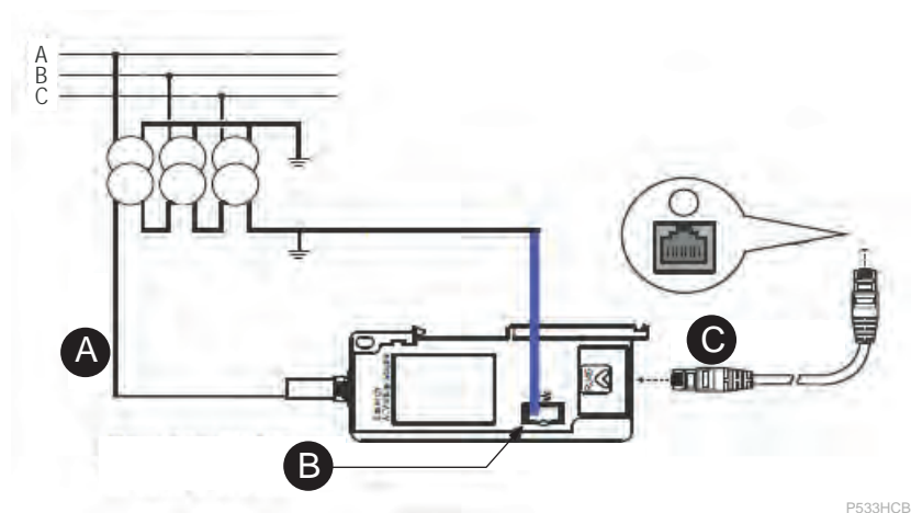
Figure 223 - Open-delta connection 1
