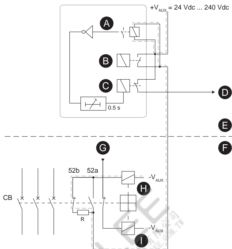
Figure 154 - Trip circuit supervision using a single digital input when the circuit breaker is in open position
