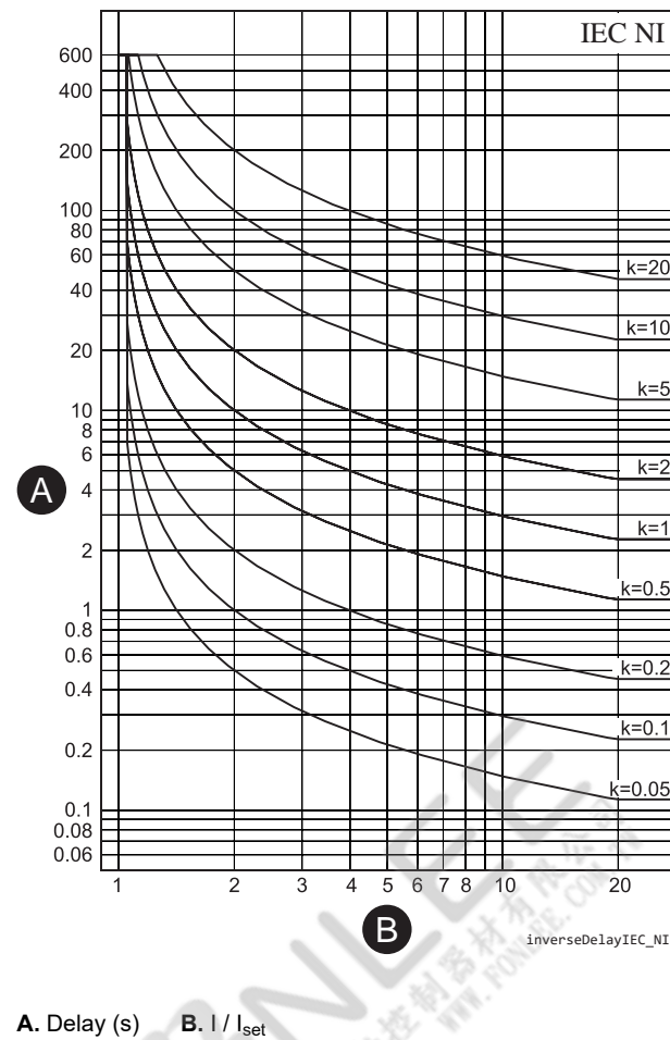
Figure 55 - IEC normal inverse delay
