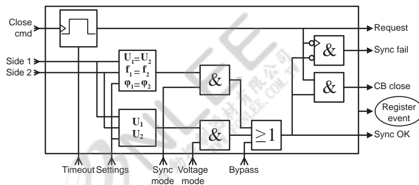
Figure 71 - Synchrocheck function
