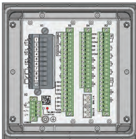
Figure 186 - Pluggable Clamp 2xLC P3Uxx-5AAA3BDA
