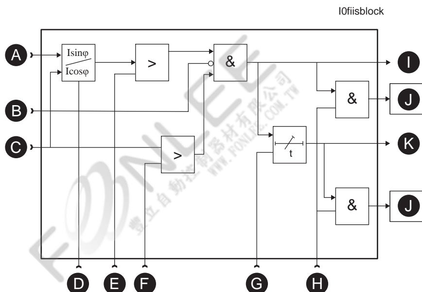
Figure 114 - Block diagram of the directional earth fault overcurrent stages I_{0\phi}> , I_{0\phi}>> , I_{0\phi}>>>
