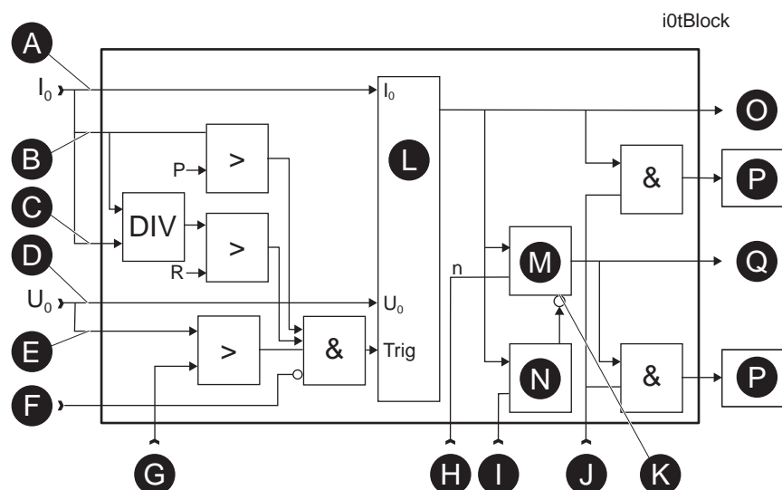
Figure 121 - Block diagram of the directional transient intermittent earth fault stage I_{0INT}>
