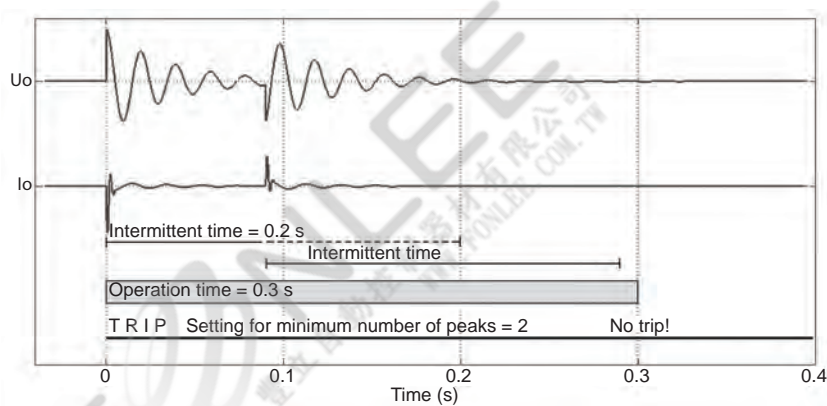
Figure 120 - Peak amount is satisfied but intermittent time comes full before operate time comes full. Stage is released.
