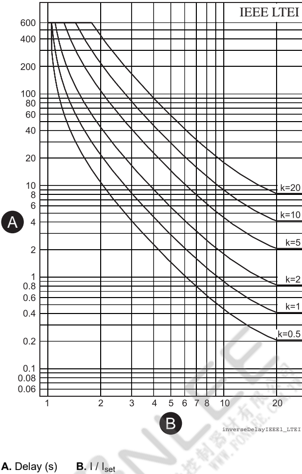
Figure 61 - ANSI/IEEE long time extremely inverse delay
