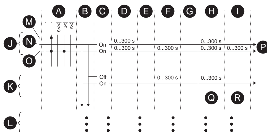
Figure 123 - Auto-recloser matrix
