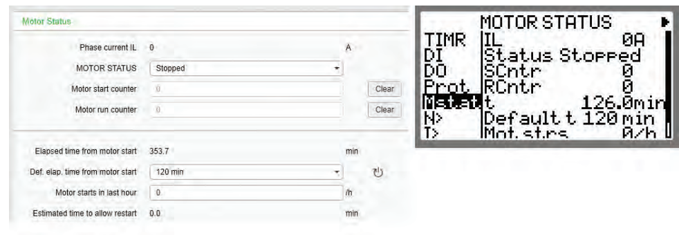
Figure 78 - Motor status via Easergy Pro and local panel
