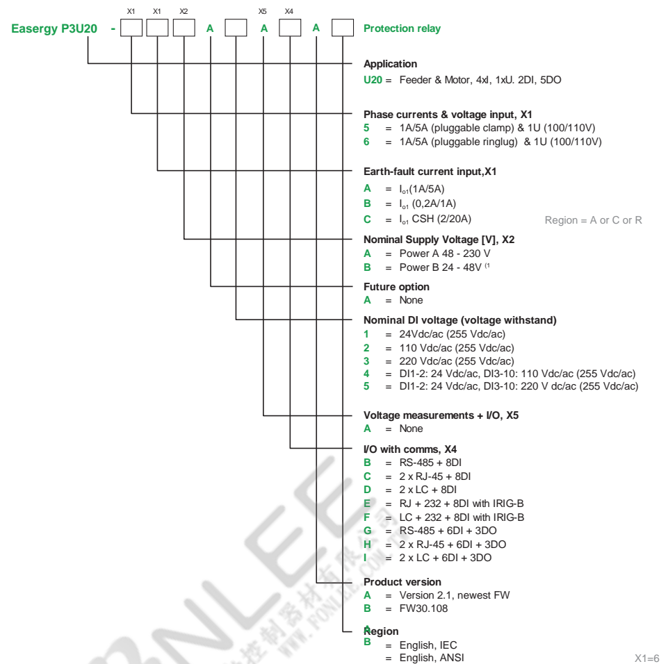
Figure 247 - P3U20 order code
