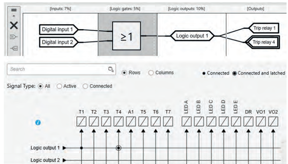
Figure 17 - Digital inputs assigned to outputs of logical operators
