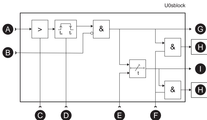
Figure 109 - Block diagram of the neutral voltage displacement stages U_0> , U_0>> , U_0>>>
