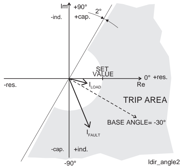
Figure 111 - Example of the directional overcurrent function's protection area
