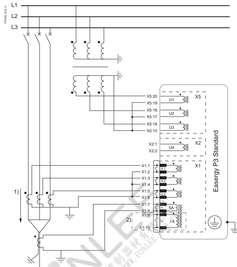
Figure 214 - 3LN voltages + 3LN currents + core balance EF
