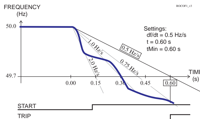
Figure 125 - An example of definite time df/dt operate time. At 0.6 s, which is the delay setting, the average slope exceeds the setting 0.5 Hz/s and a trip signal is generated.
