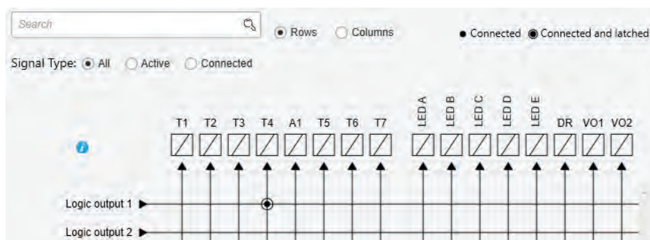
Figure 14 - Trip contacts assigned directly to outputs of logical operators
