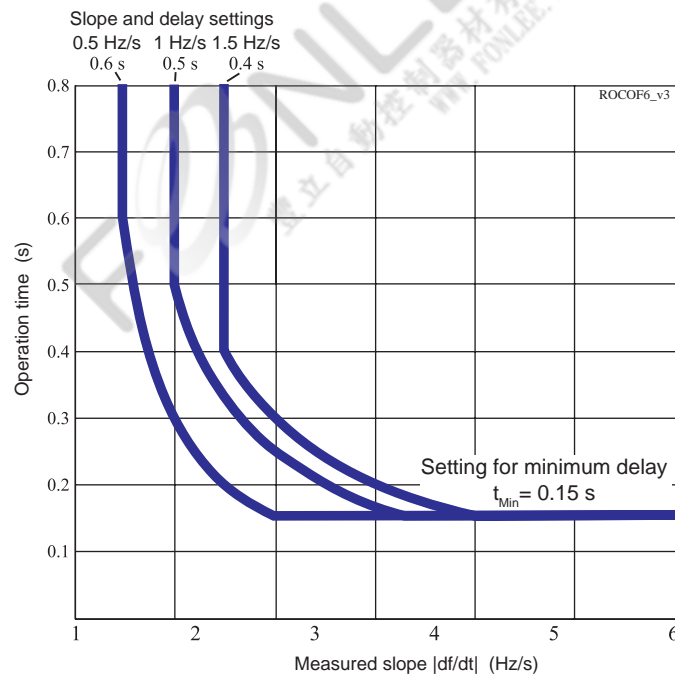
Figure 127 - Three examples of possible dependent df/dt operate time characteristics. The slope and operation delay settings define the knee points on the left. A common setting for t_{Min} has been used in these three examples. This minimum delay parameter defines the knee point positions on the right.
