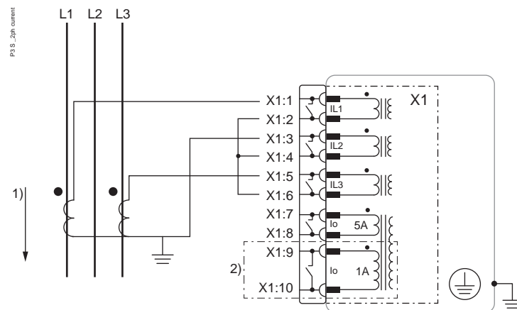
Figure 206 - Two-phase current measurement
