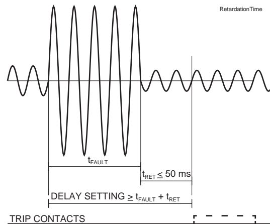
Figure 50 - Overshoot time
