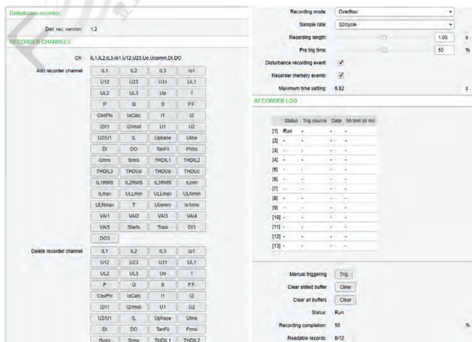
Figure 132 - Configuring the disturbance recorder
