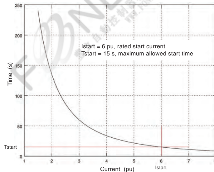
Figure 76 - Example of a dependent operate time delay of the motor start-up supervision stage
