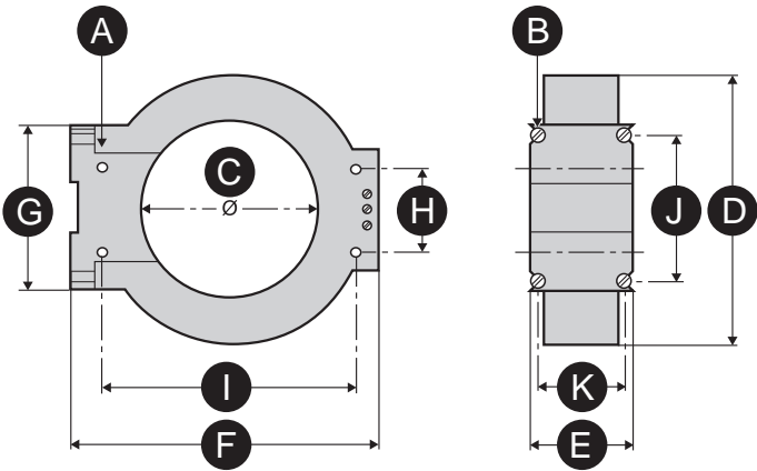
Figure 244 - Dimensions
