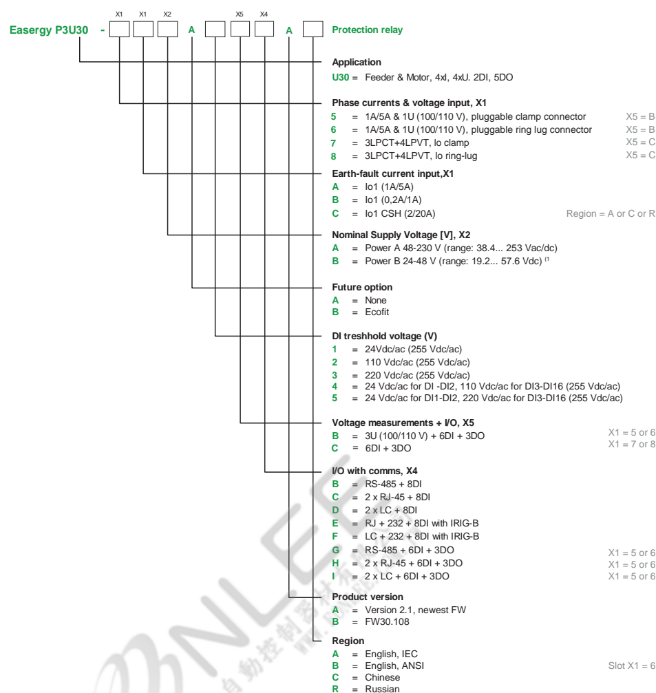
Figure 248 - P3U30 order code
