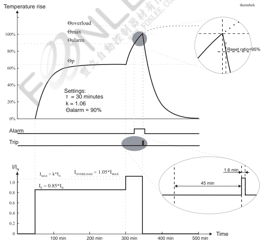
Figure 83 - Example of the thermal model behavior
