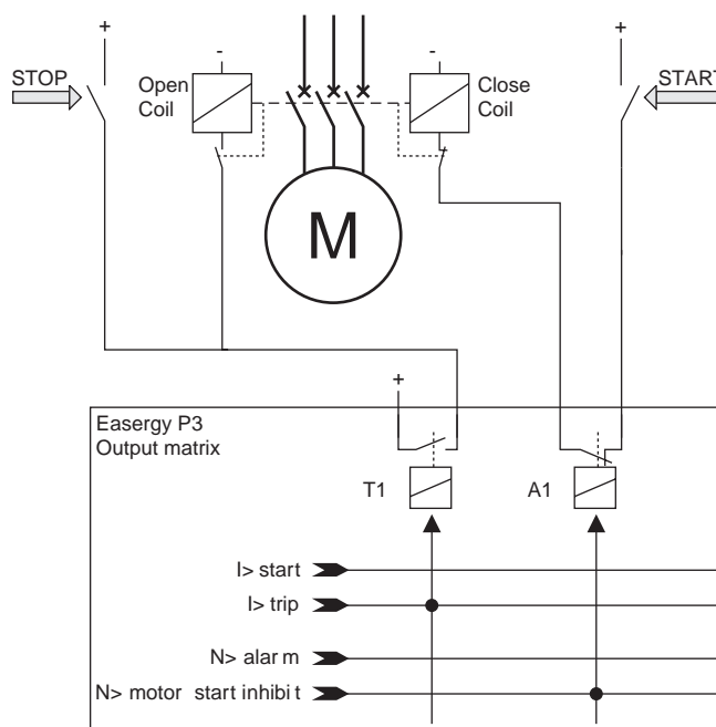
Figure 110 - Application for preventing too frequent starting using the N&gt; stage
