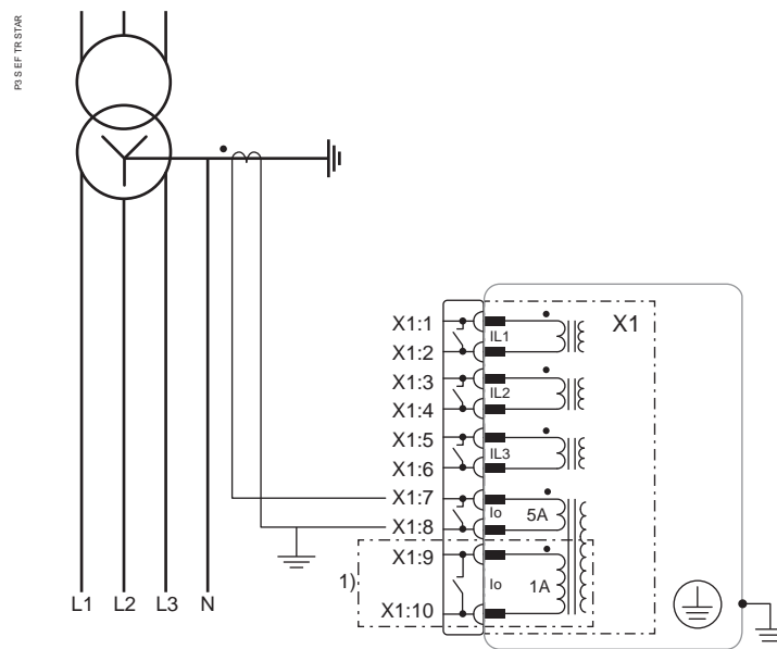
Figure 211 - Earth fault overcurrent measured from neutral earthing
