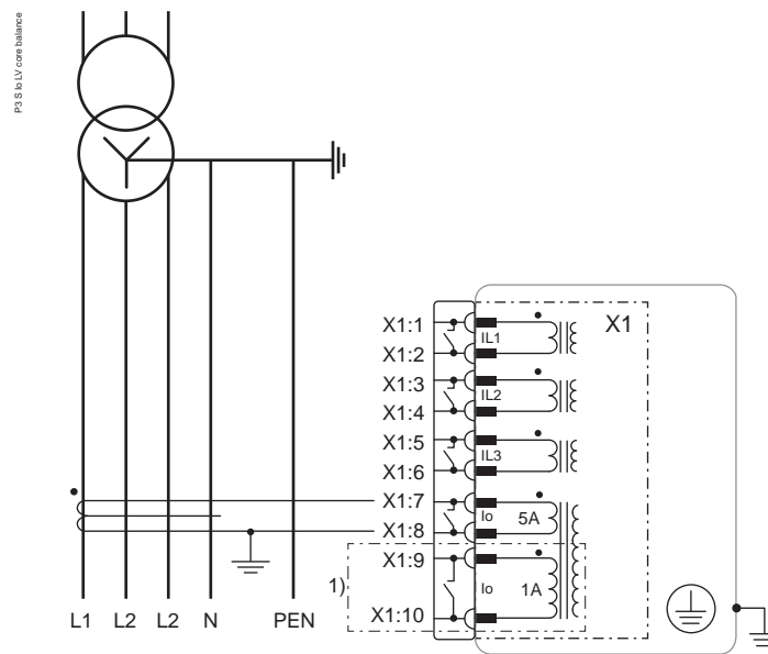
Figure 213 - Earth fault overcurrent measurement by using core balance CT
