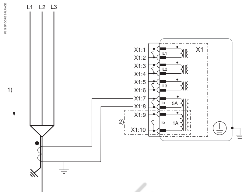
Figure 210 - Earth fault overcurrent by core balance CT
