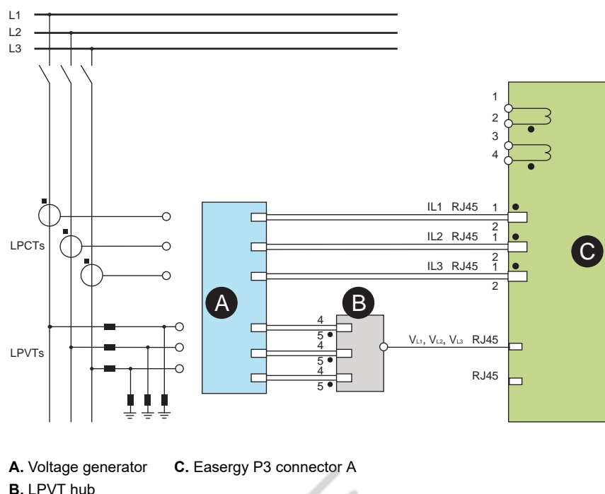
Figure 231 - Connection diagram for testing the LPIT
