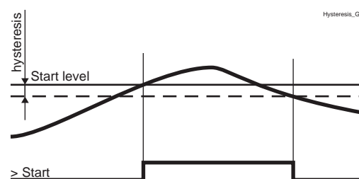
Figure 48 - Example behavior of an over-protection with hysteresis
