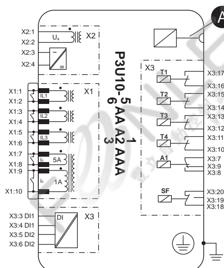
Figure 197 - P3U10 5AA A1AAA block diagram
