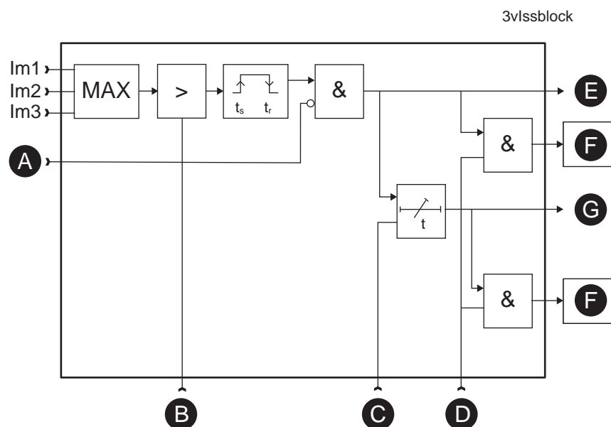
Figure 92 - Block diagram of the three-phase overcurrent stage I>> and I>>>
