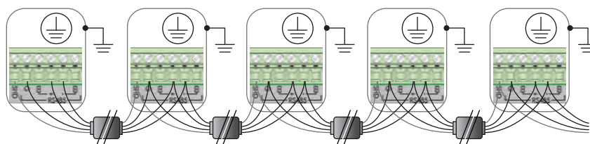
Figure 191 - RS-485 multidrop connections
