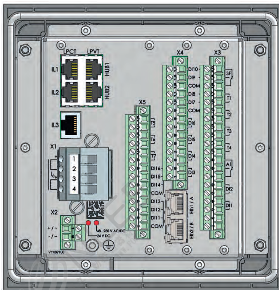
Figure 190 - P3U real panel – LPIT
