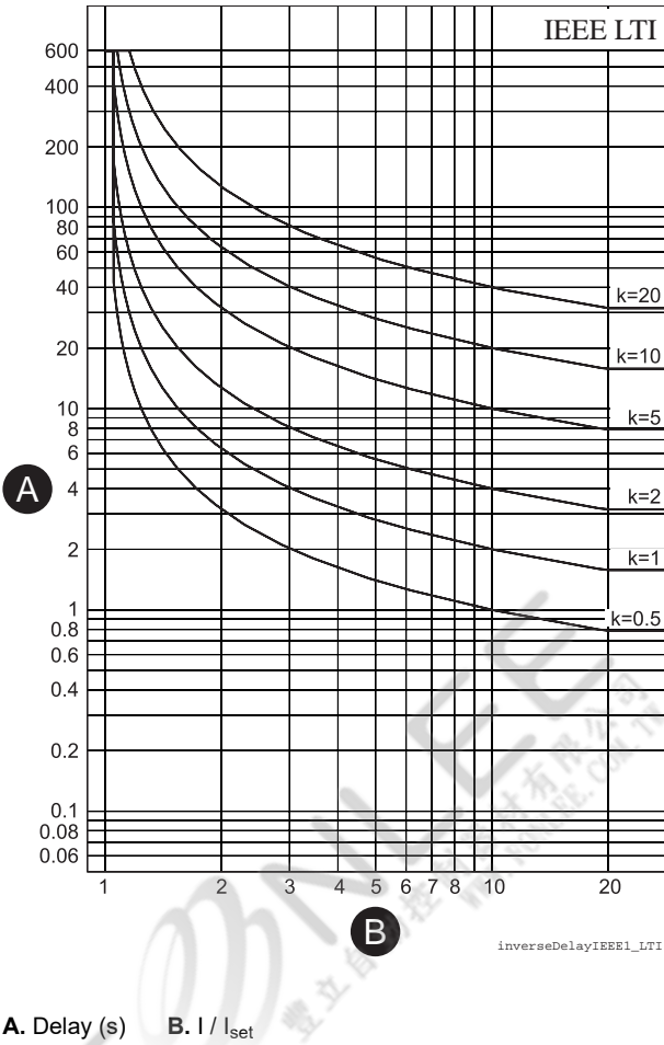
Figure 59 - ANSI/IEEE long time inverse delay
