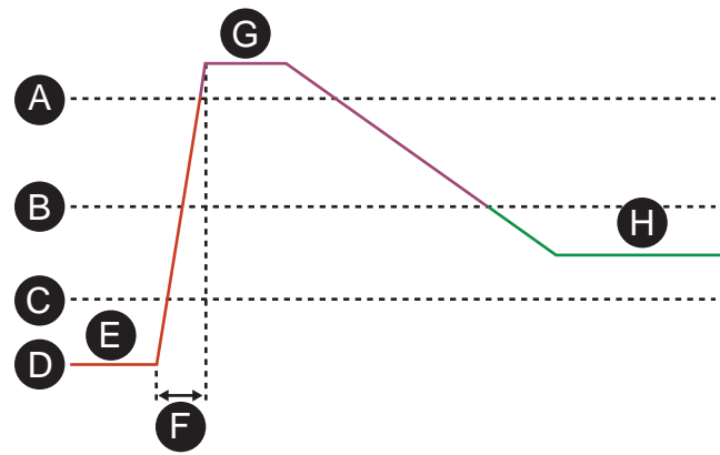
Figure 80 - Normal starting sequence
