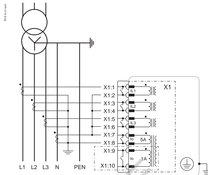
Figure 212 - Earth fault overcurrent measurement by sum of phase overcurrent and earth fault overcurrent
