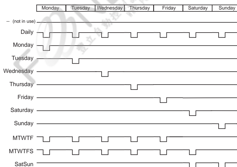
Figure 148 - Timer output sequence in different modes
