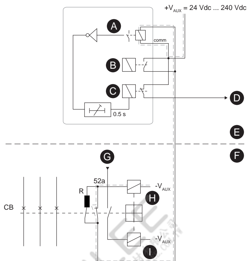
Figure 153 - Alternative connection without using circuit breaker 52b auxiliary contacts
