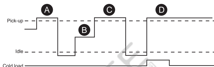
Figure 133 - Functionality of cold load / inrush current feature.
