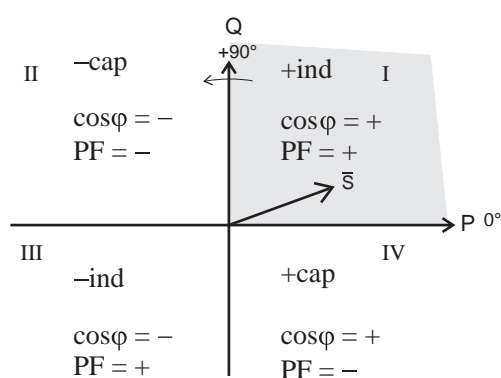
Figure 12 - Quadrants of power plane
