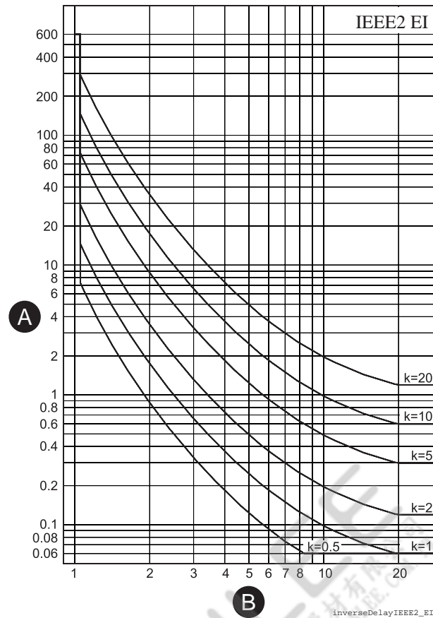
Figure 68 - IEEE2 extremely inverse delay
