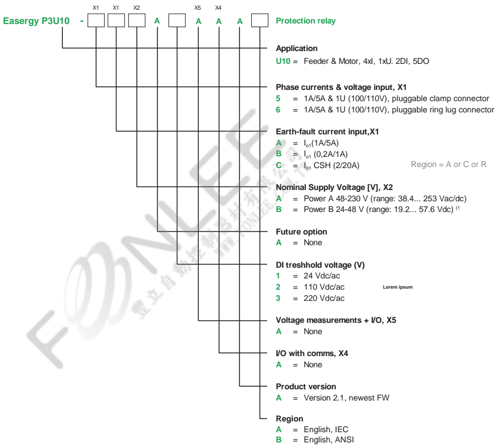
Figure 246 - P3U10 order code
