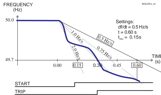
Figure 128 - An example of dependent df/dt operate time. The time to trip will be 0.3 s, although the setting is 0.6 s, because the average slope 1 Hz/s is steeper than the setting value 0.5 Hz/s.
