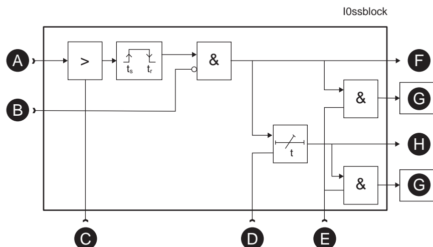
Figure 94 - Block diagram of the earth fault stages overcurrent I_0>> , I_0>>> , I_0>>>> , I_0>>>>>
