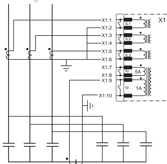
Figure 95 - Typical capacitor bank protection application with Easergy P3 relays
