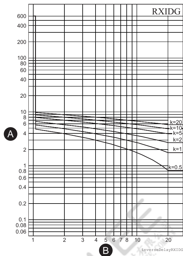
Figure 70 - RXIDG dependent delay
