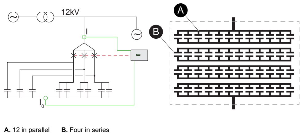
Figure 98 - 131.43 \mu\text{F} Y-Y connected capacitor bank with internal fuses
