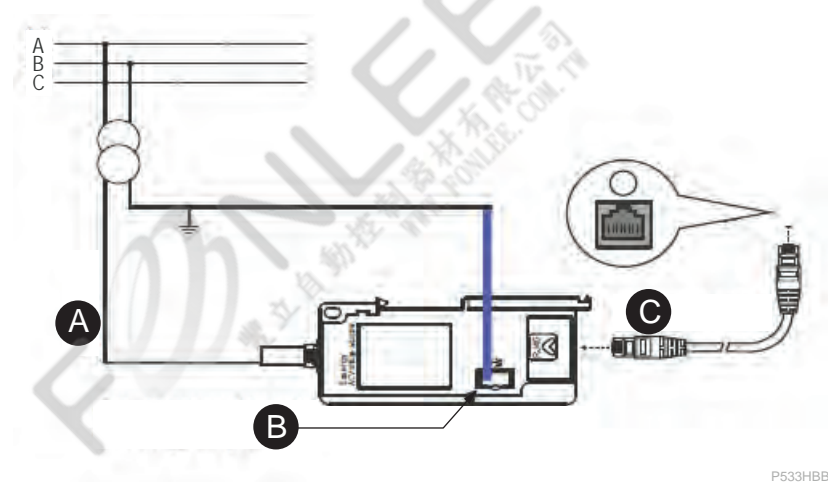
Figure 222 - 1 additional line-to-line voltage connection
