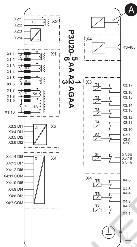
Figure 201 - P3U20 5AA A1AGAA block diagram
