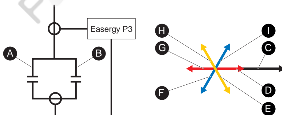
Figure 97 - How a failure in different branches of the bank affects the I_0 measurement
