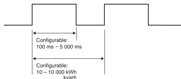
Figure 144 - Principle of energy pulses
