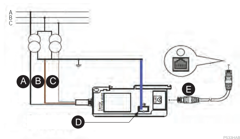
Figure 221 - 2 line-to-line voltages connection
