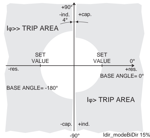
Figure 113 - Bi-directional application with two stages I_{\phi>} and I_{\phi>>}
