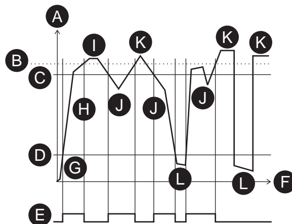
Figure 74 - Example of low-voltage self blocking
