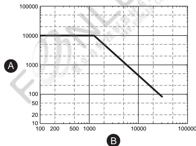
Figure 139 - Example permissible cycle diagram
