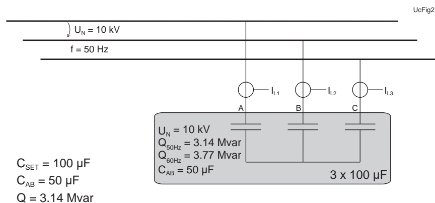
Figure 108 - Three-phase capacitor bank connected internally in wye (Y). Capacitance between phases A and B is 50 \mu\text{F} and the equivalent phase-to-neutral capacitance is 100 \mu\text{F} whose value is also used as the setting value.
