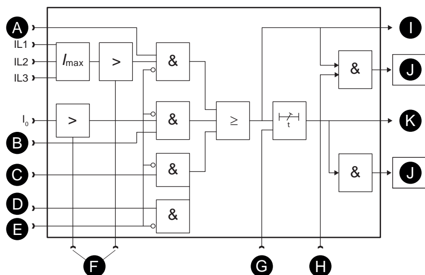
Figure 86 - Breaker failure 2 operation
