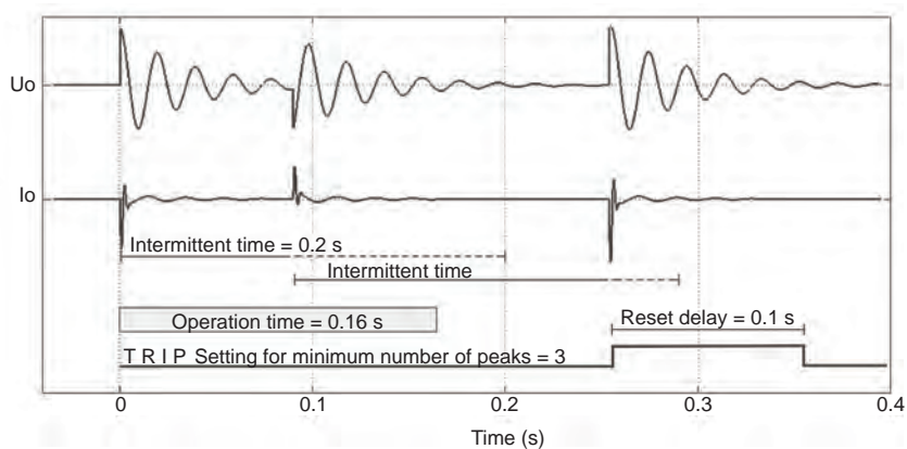
Figure 119 - Peak amount is not satisfied when operation delay comes full but last required peak comes during intermittent time. Stage issues instant trip when peak amount comes satisfied.
