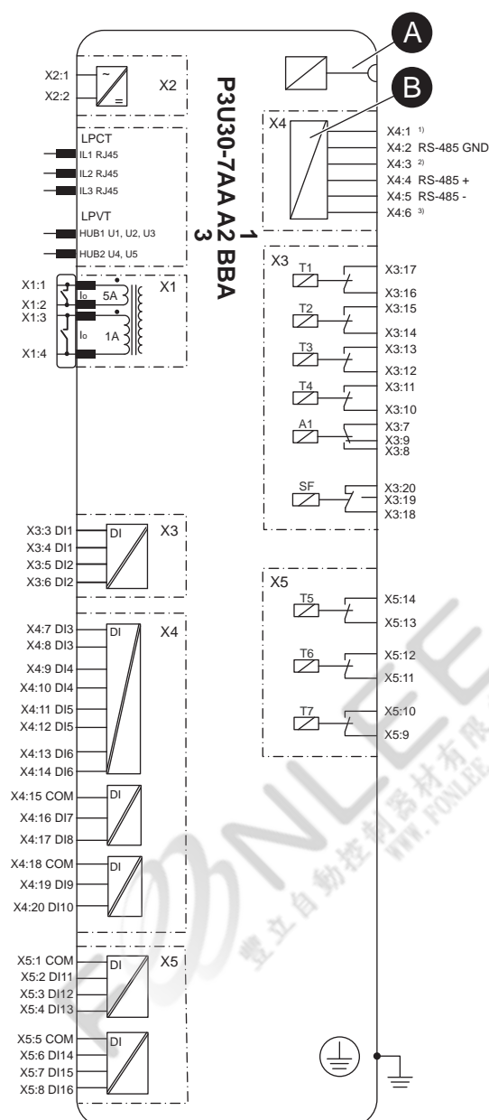
Figure 203 - P3U30 5AA A1BBA block diagram – LPIT
