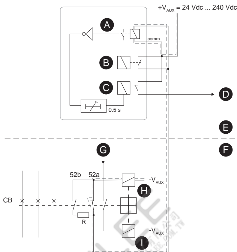
Figure 152 - Trip circuit supervision using a single digital input and an external resistor R
