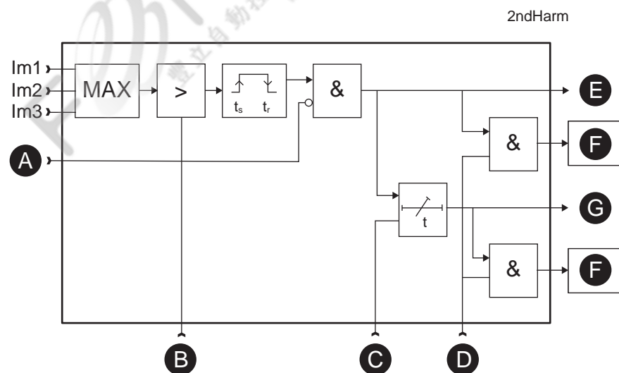
Figure 122 - Block diagram of the magnetizing inrush dection stage
