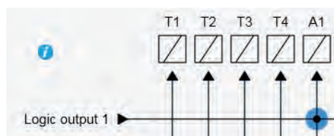
Figure 162 - An example of output matrix configuration for trip circuit supervision with two digital inputs
