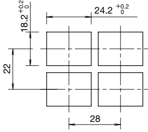
长方形 (LB8P/LB8MP 型)
