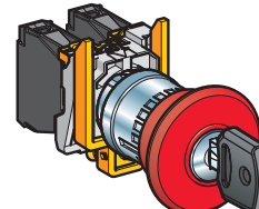
Key release (EN/ISO 13850) XB4BS9445 see page 44
