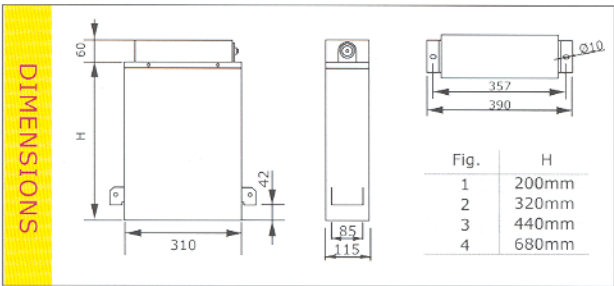
RATING AND DIMENSIONS TABLE
