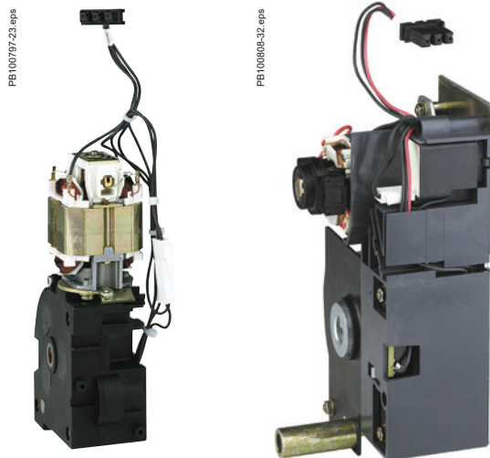
Electric motor MCH for MasterPact NT.
