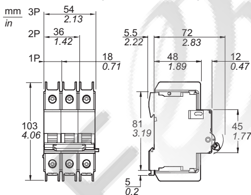
C60BP Tunnel terminal
