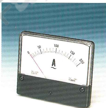
TH-120S Model: TH-120S Size: 120×100×40mm Panel cut-out Ø : 70mm
