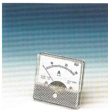
TH-65 Model: TH-65 Size: 66×66×40mm Panel cut-out Ø : 52mm
