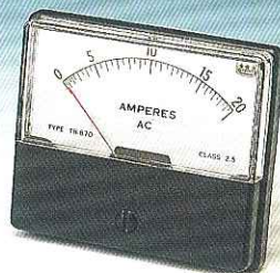
TH-670 Model: TH-670 Size: 60×70×40mm Panel cut-out Ø : 52mm
