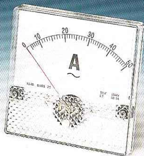
YS-10 Model: YS-10 Size: 100×100×50mm Panel cut-out Ø : 84mm
