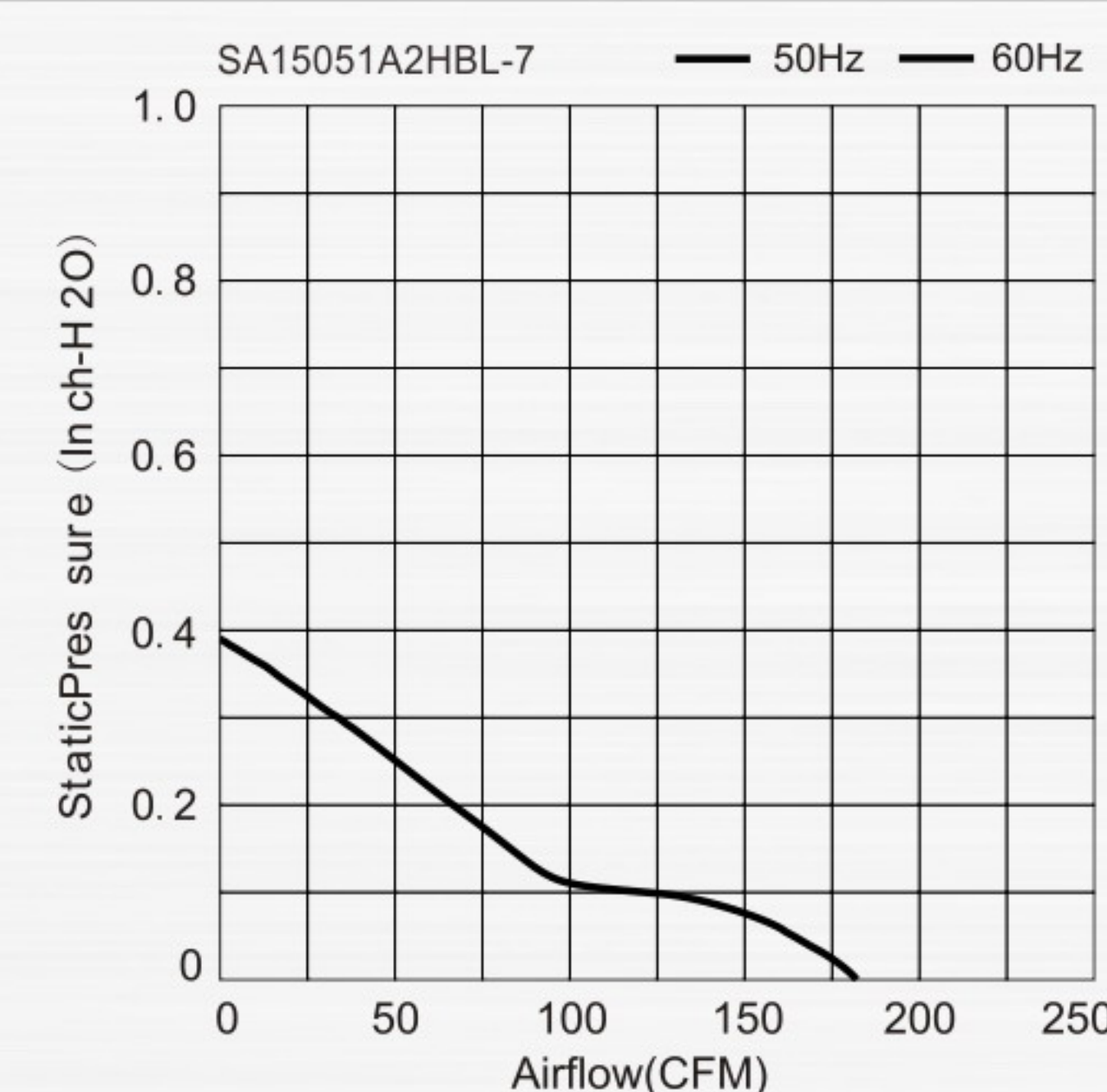
> Air Flow-Static Pressure Characteristics 氣流和靜壓特性
