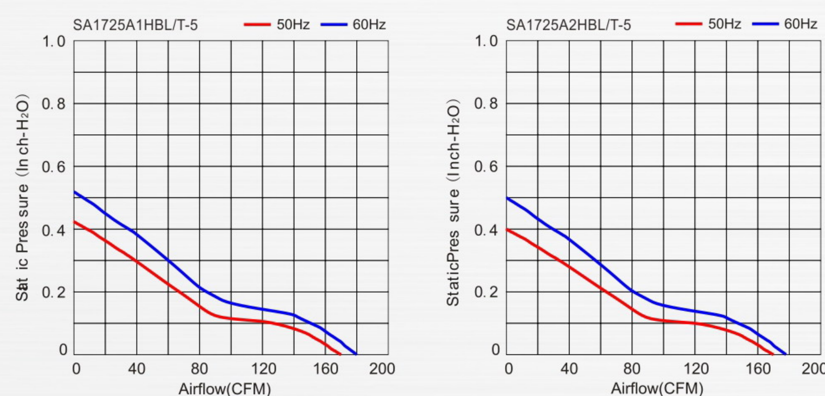
> Air Flow-Static Pressure Characteristics 氣流和靜壓特性
