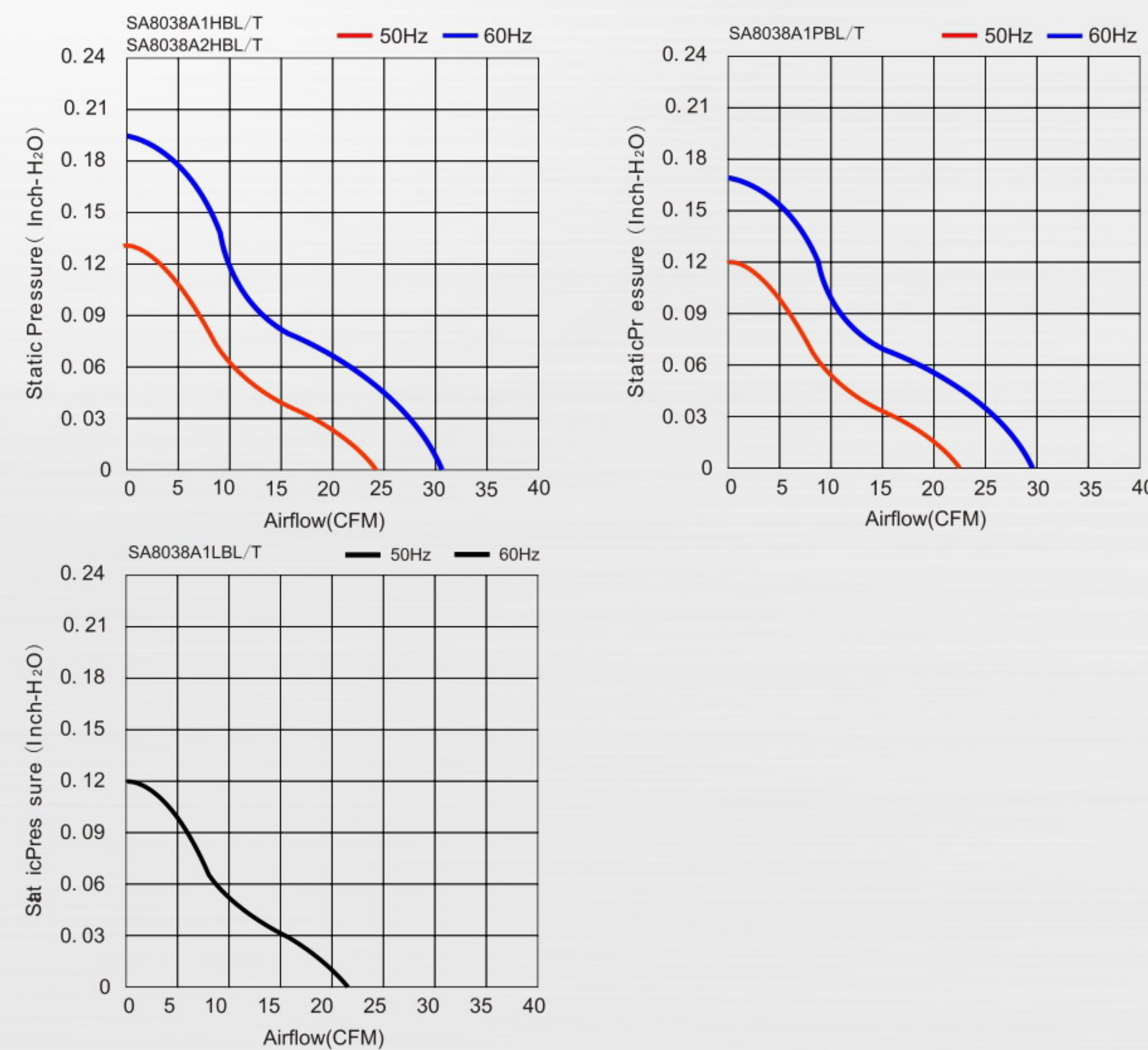
> Air Flow-Static Pressure Characteristics 氣流和靜壓特性
