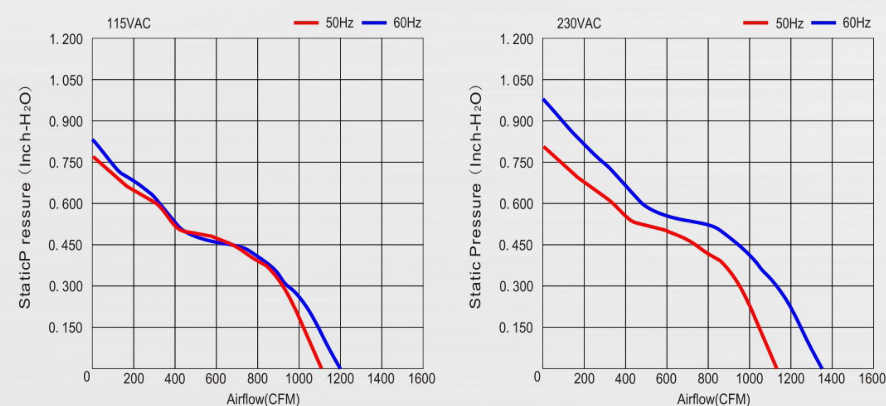
> Air Flow-Static Pressure Characteristics 氣流和靜壓特性
