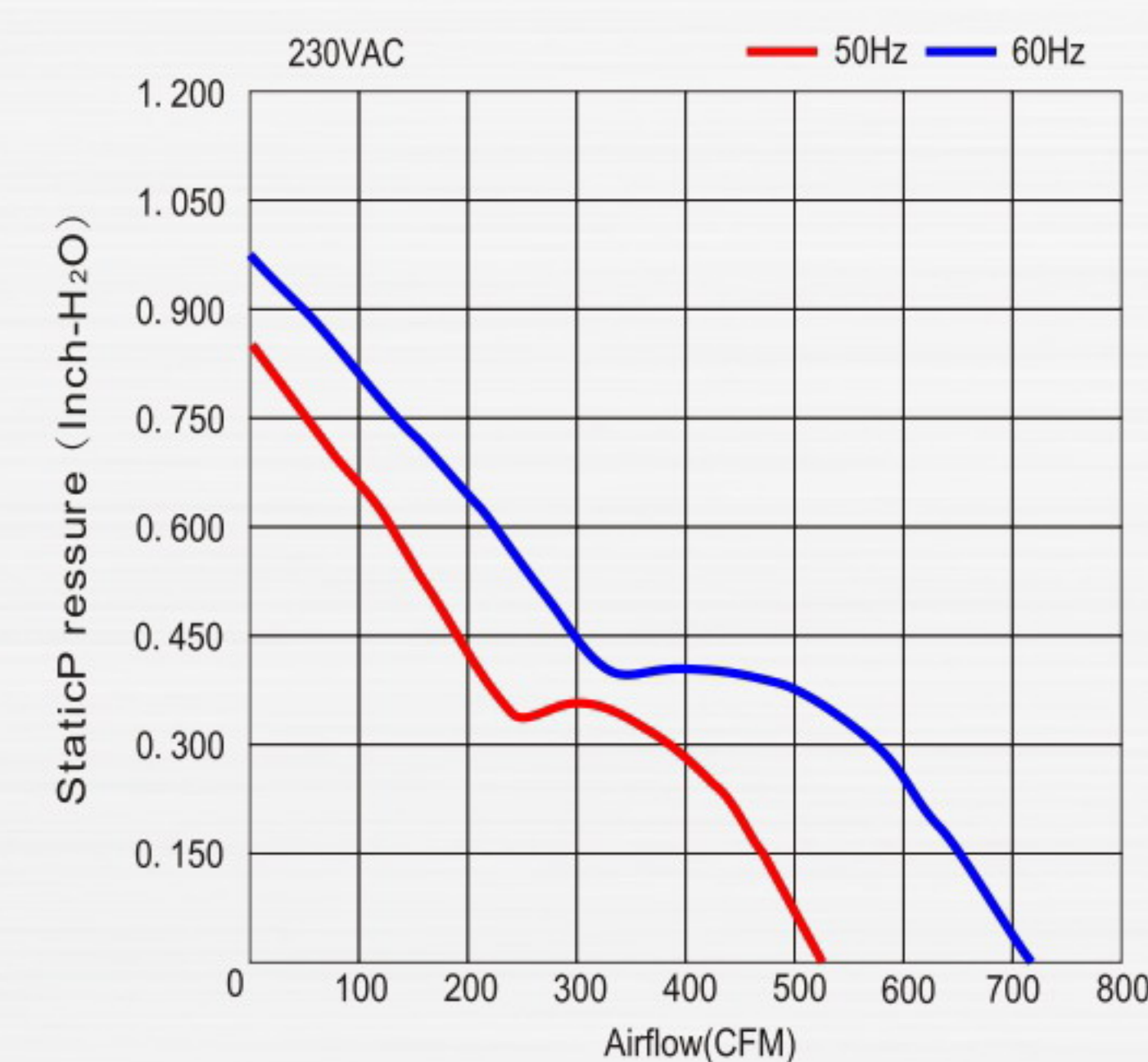
> Air Flow-Static Pressure Characteristics 氣流和靜壓特性
