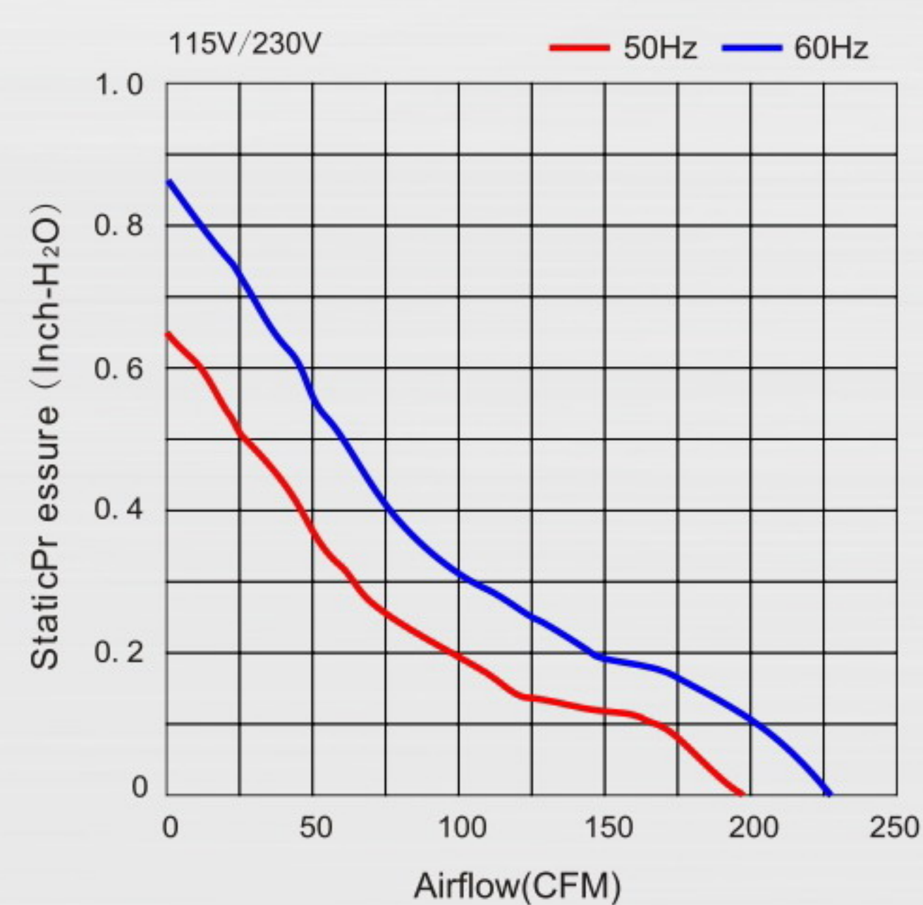
> Air Flow-Static Pressure Characteristics 氣流和靜壓特性
