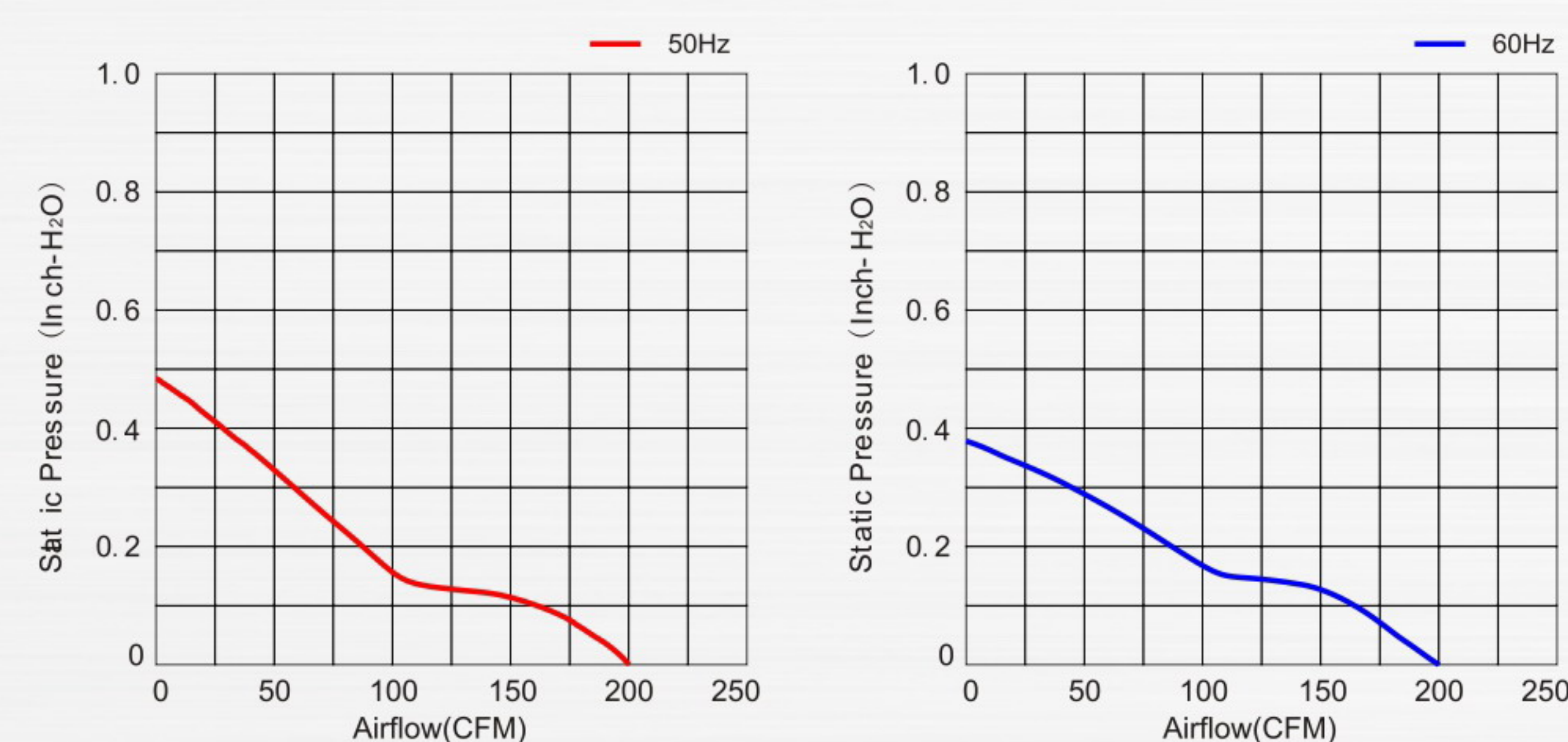
> Air Flow-Static Pressure Characteristics 氣流和靜壓特性
